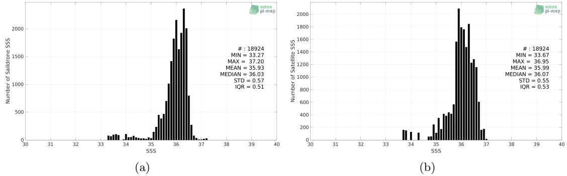
Figure 2: Histograms of SSS from Saildrone (a) and CCI SSS L4 Merged-OI v3.2 - 7-day running (ESA) (b) considering all match-up pairs per bins of 0.1 over the Tropical Atlantic Ocean Pi-MEP region and for the full satellite product period.
