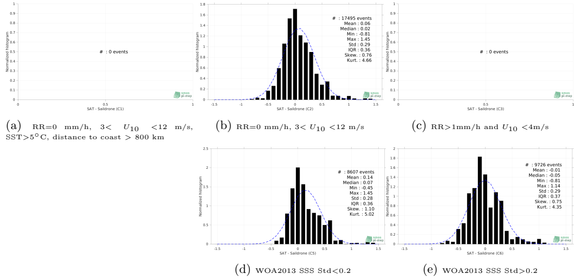
Figure 13: Normalized histogram of \Delta SSS (CCI SSS L4 Merged-OI v3.2 - 7-day running (ESA) - Saildrone) for 5 different subdatasets corresponding to: RR=0 mm/h, 3 < U_{10} < 12 m/s, SST > 5°C, distance to coast > 800 km (a), RR=0 mm/h, 3 < U_{10} < 12 m/s (b), RR > 1mm/h and U_{10} < 4 m/s (c), WOA2013 SSS Std < 0.2 (d), WOA2013 SSS Std > 0.2 (e).
