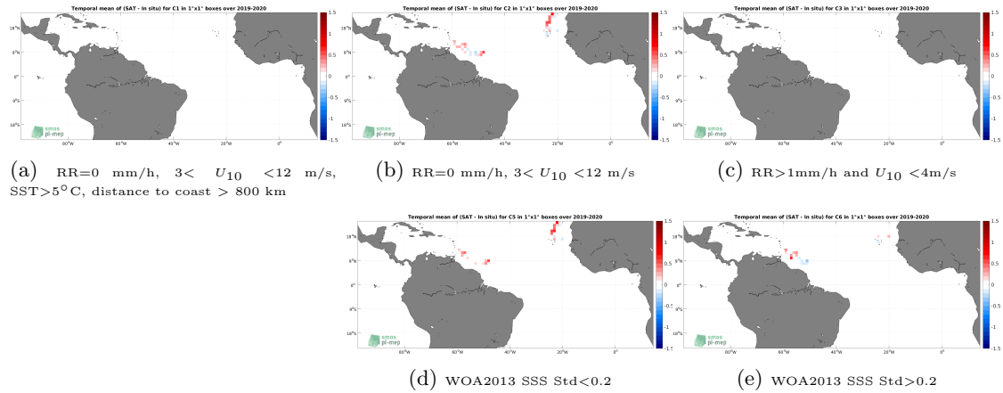
Figure 12: Temporal mean gridded over spatial boxes of size 1^\circ \times 1^\circ of \Delta SSS (CCI SSS L4 Merged-OI v3.2 - 7-day running (ESA) - Sairdrone) for 5 different subdatasets corresponding to:RR=0 mm/h, 3 < U_{10} < 12 m/s, SST >5^\circ C, distance to coast > 800 km (a), RR=0 mm/h, 3 < U_{10} < 12 m/s (b), RR >1 mm/h and U_{10} < 4 m/s (c), WOA2013 SSS Std <0.2 (d), WOA2013 SSS Std >0.2 (e).
