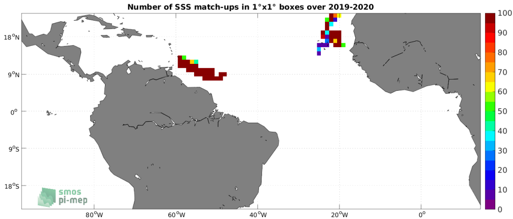
Figure 4: Number of SSS match-ups between Saifdrone SSS and the CCI SSS L4 Merged-OI v3.2 - 7-day running (ESA) SSS product for the Tropical Atlantic Ocean Pi-MEP region over 1^\circ \times 1^\circ boxes and for the full satellite product period.
