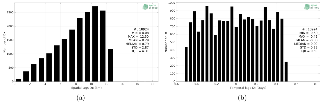
Figure 5: Histograms of the spatial (a) and temporal (b) lags between the location/time of the Saifdrone measurement and the date of the corresponding CCI SSS L4 Merged-OI v3.2 - 7-day running (ESA) SSS pixel.
