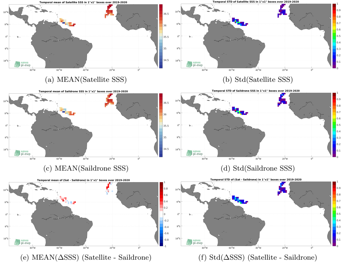
Figure 6: Temporal mean (left) and Std (right) of SSS from CCI SSS L4 Merged-OI v3.2 - 7-day running (ESA) (top), Saildrone (middle), and of \Delta SSS (Satellite - Saildrone). Only match-up pairs are used to generate these maps.
