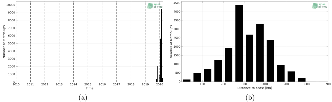
Figure 1: Number of match-ups between Saildrone and CCI SSS L4 Merged-OI v3.2 - 7-day running (ESA) SSS as a function of time (a) and as function of the distance to coast (b) over the Tropical Atlantic Ocean Pi-MEP region and for the full satellite product period.
