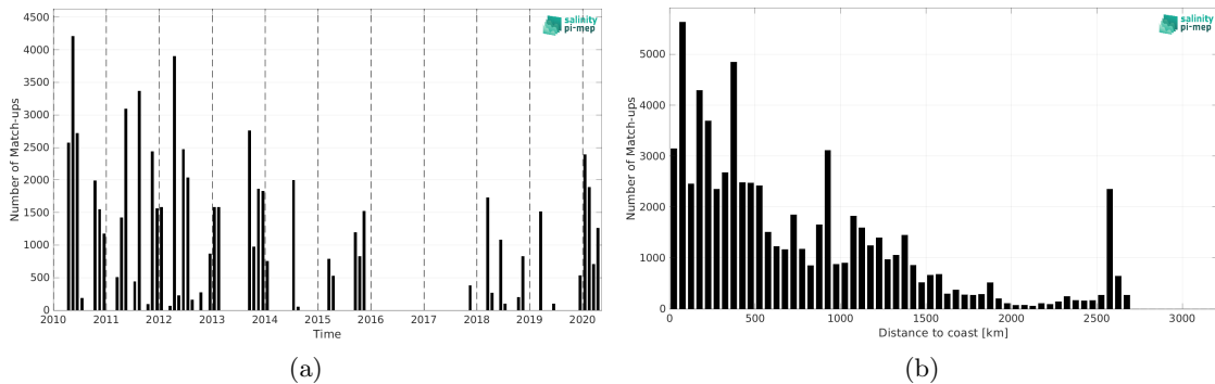
Figure 1: Number of match-ups between TSG (SAMOS) and CCI SSS L4 Merged-OI v3.2 - 30-day running (ESA) SSS as a function of time (a) and as function of the distance to coast (b) over the Tropical Atlantic Ocean Pi-MEP region and for the full satellite product period.
