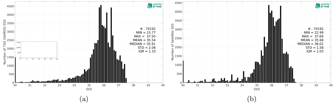
Figure 2: Histograms of SSS from TSG (SAMOS) (a) and CCI SSS L4 Merged-OI v3.2 - 30-day running (ESA) (b) considering all match-up pairs per bins of 0.1 over the Tropical Atlantic Ocean Pi-MEP region and for the full satellite product period.
