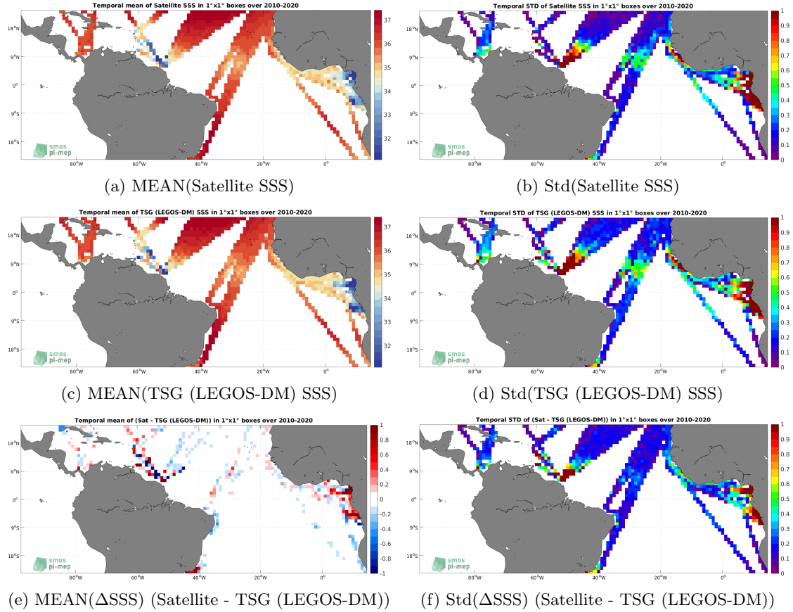
Figure 6: Temporal mean (left) and Std (right) of SSS from CCI SSS L4 Merged-OI v3.2 - 30-day running (ESA) (top), TSG (LEGOS-DM) (middle), and of \Delta\text{SSS} (Satellite - TSG (LEGOS-DM)). Only match-up pairs are used to generate these maps.
