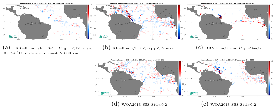
Figure 12: Temporal mean gridded over spatial boxes of size 1^\circ \times 1^\circ of \Delta\text{SSS} (CCI SSS L4 Merged-OI v3.2 - 30-day running (ESA) - TSG (GOSUD-Research-vessel)) for 5 different subdatasets corresponding to:RR=0 mm/h, 3 < U_{10} < 12 m/s, SST >5^\circ\text{C} , distance to coast > 800 km (a), RR=0 mm/h, 3 < U_{10} < 12 m/s (b), RR >1 mm/h and U_{10} < 4 m/s (c), WOA2013 SSS Std <0.2 (d), WOA2013 SSS Std >0.2 (e).
