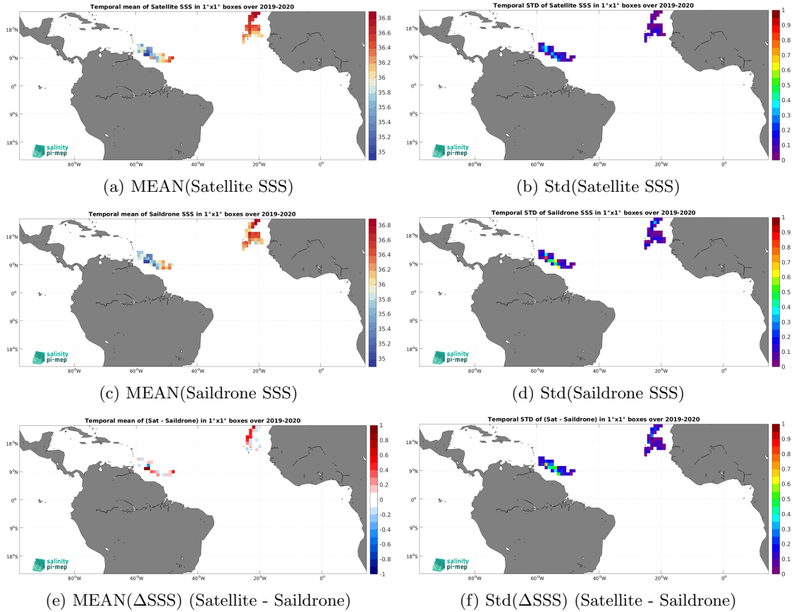
Figure 6: Temporal mean (left) and Std (right) of SSS from CCI SSS L4 Merged-OI v3.2 - 30-day running (ESA) (top), Saildrone (middle), and of \Delta SSS (Satellite - Saildrone). Only match-up pairs are used to generate these maps.
