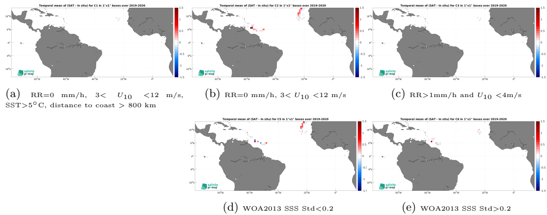
Figure 12: Temporal mean gridded over spatial boxes of size 1^\circ \times 1^\circ of \Delta\text{SSS} (CCI SSS L4 Merged-OI v3.2 - 30-day running (ESA) - Saildrone) for 5 different subdatasets corresponding to:RR=0 mm/h, 3 < U_{10} < 12 m/s, SST >5^\circ\text{C} , distance to coast > 800 km (a), RR=0 mm/h, 3 < U_{10} < 12 m/s (b), RR >1 mm/h and U_{10} < 4 m/s (c), WOA2013 SSS Std <0.2 (d), WOA2013 SSS Std >0.2 (e).
