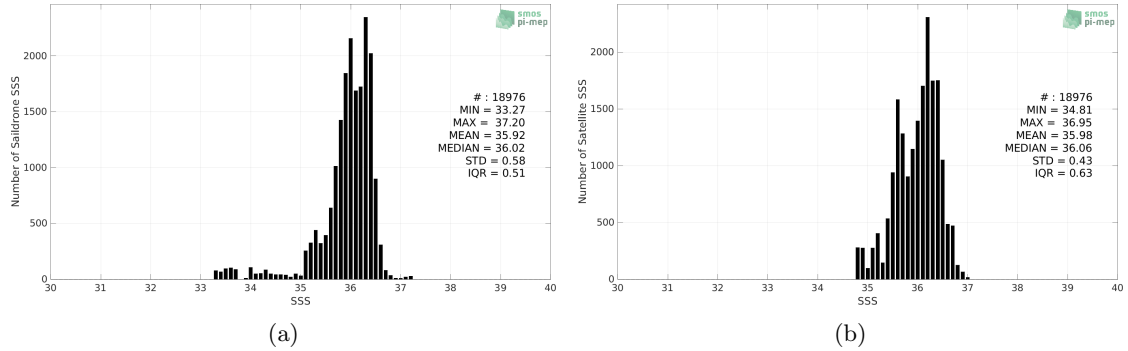
Figure 2: Histograms of SSS from Saildrone (a) and CCI SSS L4 Merged-OI v3.2 - 30-day running (ESA) (b) considering all match-up pairs per bins of 0.1 over the Tropical Atlantic Ocean Pi-MEP region and for the full satellite product period.
