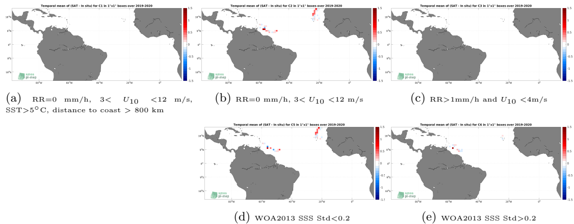
Figure 12: Temporal mean gridded over spatial boxes of size 1^\circ \times 1^\circ of \Delta SSS (CCI SSS L4 Merged-OI v3.2 - 30-day running (ESA) - Saildrone) for 5 different subdatasets corresponding to:RR=0 mm/h, 3 < U_{10} < 12 m/s, SST >5^\circ\text{C} , distance to coast > 800 km (a), RR=0 mm/h, 3 < U_{10} < 12 m/s (b), RR >1 mm/h and U_{10} < 4 m/s (c), WOA2013 SSS Std <0.2 (d), WOA2013 SSS Std >0.2 (e).
