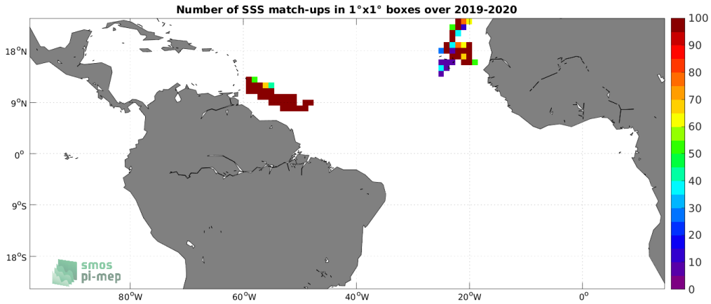
Figure 4: Number of SSS match-ups between Saildrone SSS and the CCI SSS L4 Merged-OI v3.2 - 30-day running (ESA) SSS product for the Tropical Atlantic Ocean Pi-MEP region over 1^\circ \times 1^\circ boxes and for the full satellite product period.
