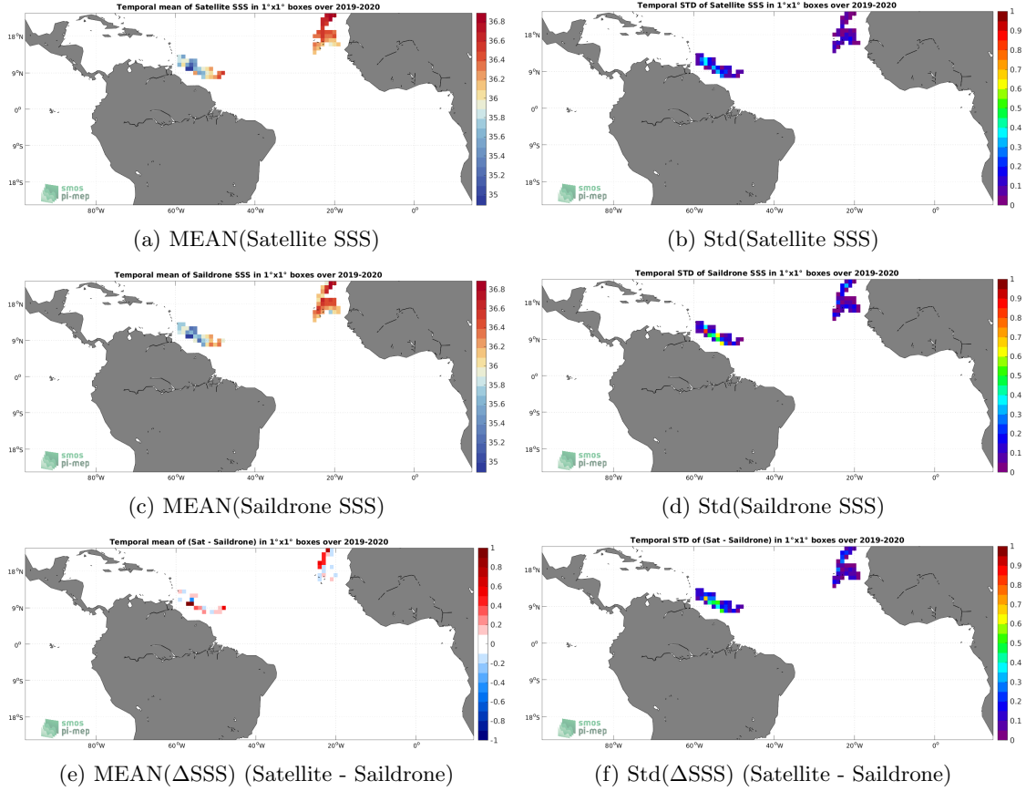
Figure 6: Temporal mean (left) and Std (right) of SSS from CCI SSS L4 Merged-OI v3.2 - 30-day running (ESA) (top), Saildrone (middle), and of \Delta\text{SSS} (Satellite - Saildrone). Only match-up pairs are used to generate these maps.
