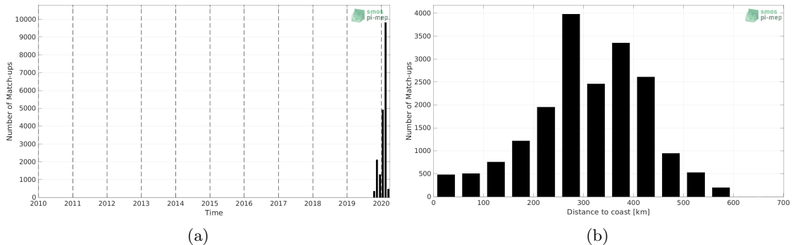
Figure 1: Number of match-ups between Saildrone and CCI SSS L4 Merged-OI v3.2 - 30-day running (ESA) SSS as a function of time (a) and as function of the distance to coast (b) over the Tropical Atlantic Ocean Pi-MEP region and for the full satellite product period.
