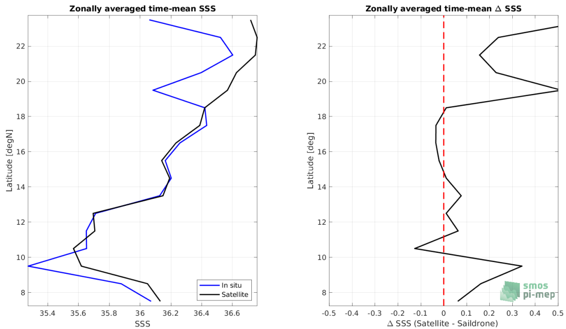
Figure 8: Left panel: Zonal mean SSS from CCI SSS L4 Merged-OI v3.2 - 30-day running (ESA) satellite product (black) and from SAILDRONE (blue). Right panel: Zonal mean of \Delta SSS (Satellite - SAILDRONE) for all the collected Pi-MEP match-up pairs estimated over the full satellite product period.
