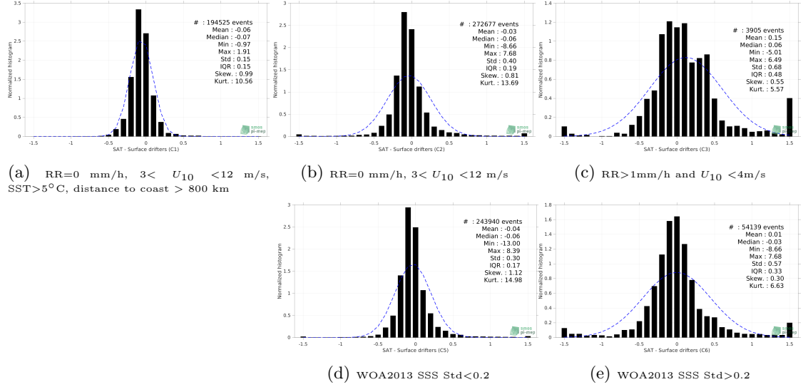
Figure 12: Normalized histogram of \Delta SSS (CCI SSS L4 Merged-OI v3.2 - 30-day running (ESA) - Surface drifters) for 5 different subdatasets corresponding to: RR=0 mm/h, 3 < U_{10} < 12 m/s, SST>5°C, distance to coast > 800 km (a), RR=0 mm/h, 3 < U_{10} < 12 m/s (b), RR>1mm/h and U_{10} < 4 m/s (c), WOA2013 SSS Std<0.2 (d), WOA2013 SSS Std>0.2 (e).
