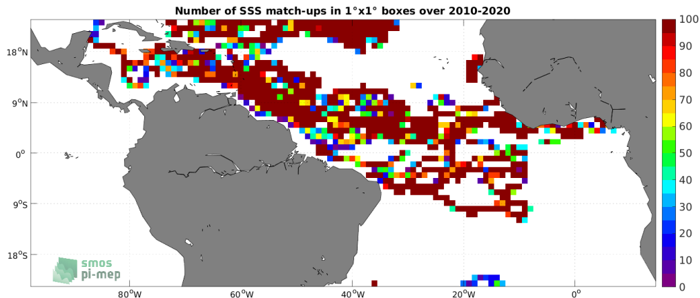
Figure 3: Number of SSS match-ups between Surface drifters SSS and the CCI SSS L4 Merged-OI v3.2 - 30-day running (ESA) SSS product for the Tropical Atlantic Ocean Pi-MEP region over 1^\circ \times 1^\circ boxes and for the full satellite product period.
