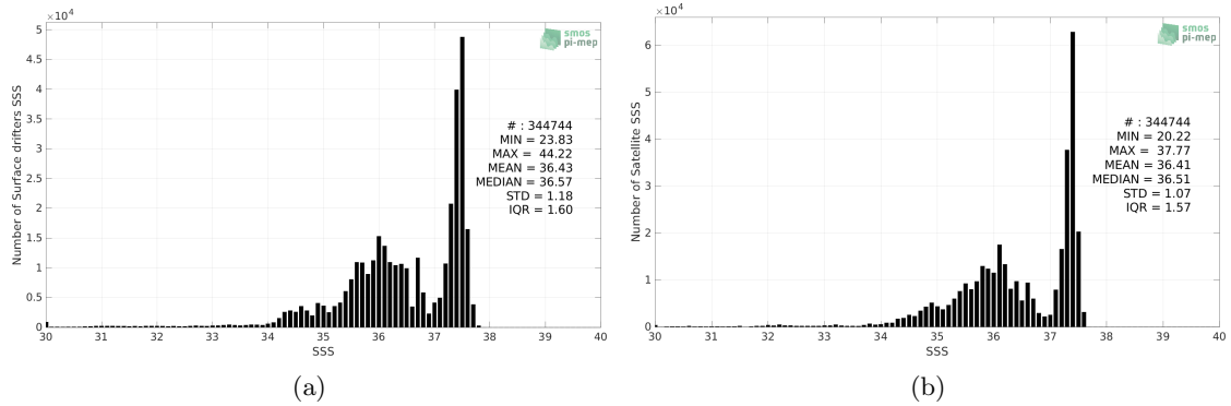
Figure 2: Histograms of SSS from Surface drifters (a) and CCI SSS L4 Merged-OI v3.2 - 30-day running (ESA) (b) considering all match-up pairs per bins of 0.1 over the Tropical Atlantic Ocean Pi-MEP region and for the full satellite product period.
