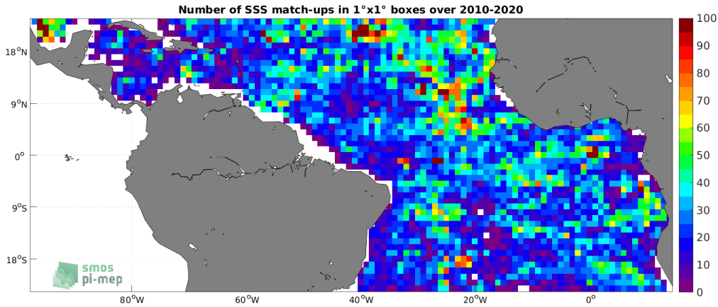
Figure 4: Number of SSS match-ups between Argo SSS and the CCI SSS L4 Merged-OI v3.2 - 30-day running (ESA) SSS product for the Tropical Atlantic Ocean Pi-MEP region over 1^\circ \times 1^\circ boxes and for the full satellite product period.
