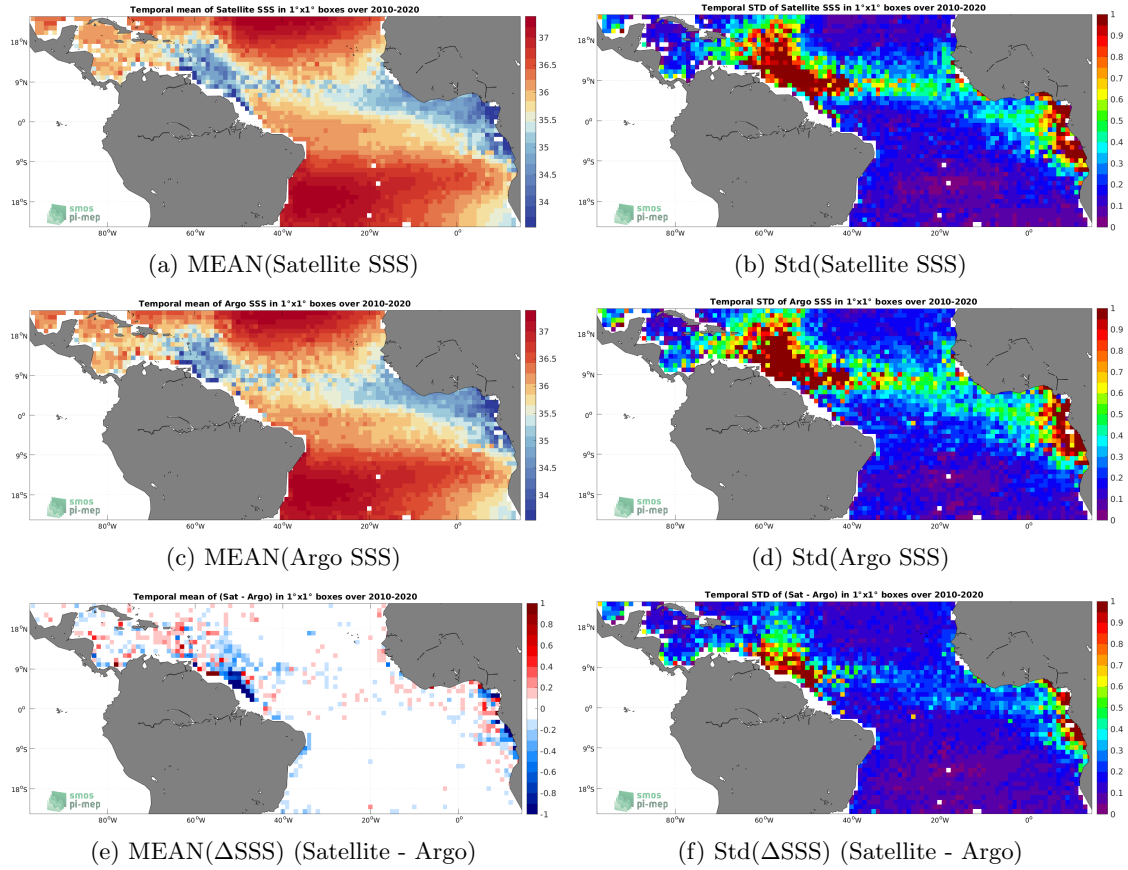
Figure 6: Temporal mean (left) and Std (right) of SSS from CCI SSS L4 Merged-OI v3.2 - 30-day running (ESA) (top), Argo (middle), and of \Delta\text{SSS} (Satellite - Argo). Only match-up pairs are used to generate these maps.
