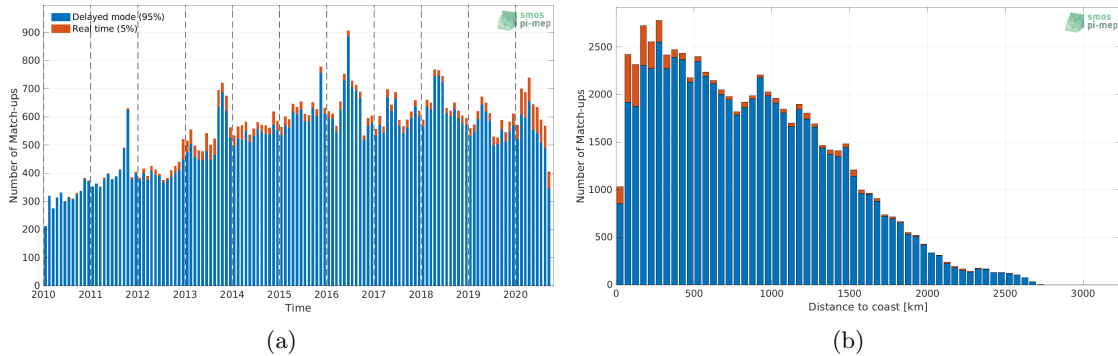
Figure 1: Number of match-ups between Argo and CCI SSS L4 Merged-OI v3.2 - 30-day running (ESA) SSS as a function of time (a) and as function of the distance to coast (b) over the Tropical Atlantic Ocean Pi-MEP region and for the full satellite product period.
