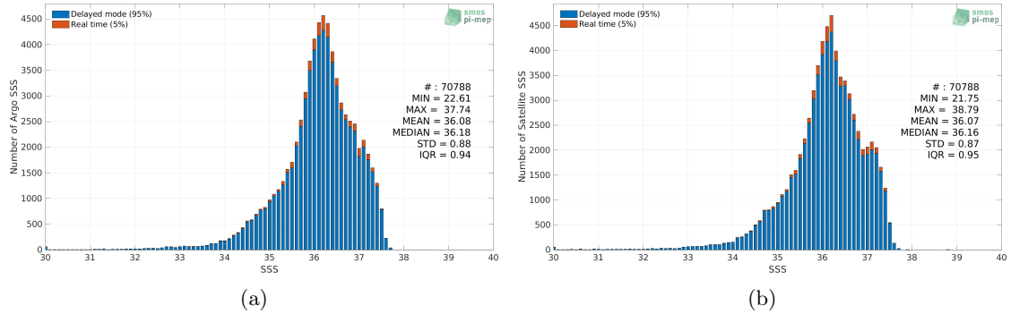
Figure 2: Histograms of SSS from Argo (a) and CCI SSS L4 Merged-OI v3.2 - 30-day running (ESA) (b) considering all match-up pairs per bins of 0.1 over the Tropical Atlantic Ocean Pi-MEP region and for the full satellite product period.
