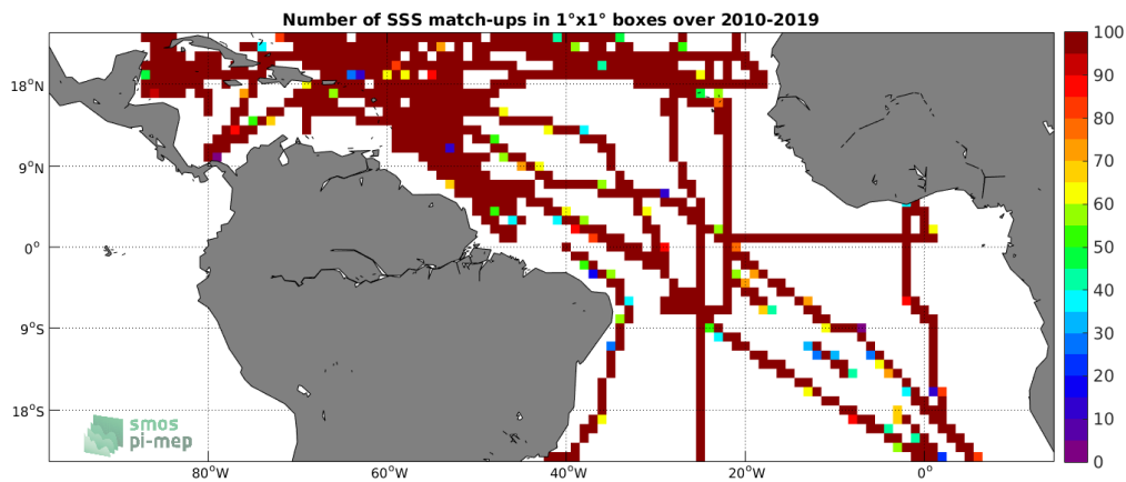
Figure 4: Number of SSS match-ups between TSG (SAMOS) SSS and the CCI L4 Merged-OI v2.31 - 7-day running (ESA) SSS product for the Tropical Atlantic Ocean Pi-MEP region over 1^\circ \times 1^\circ boxes and for the full satellite product period.
