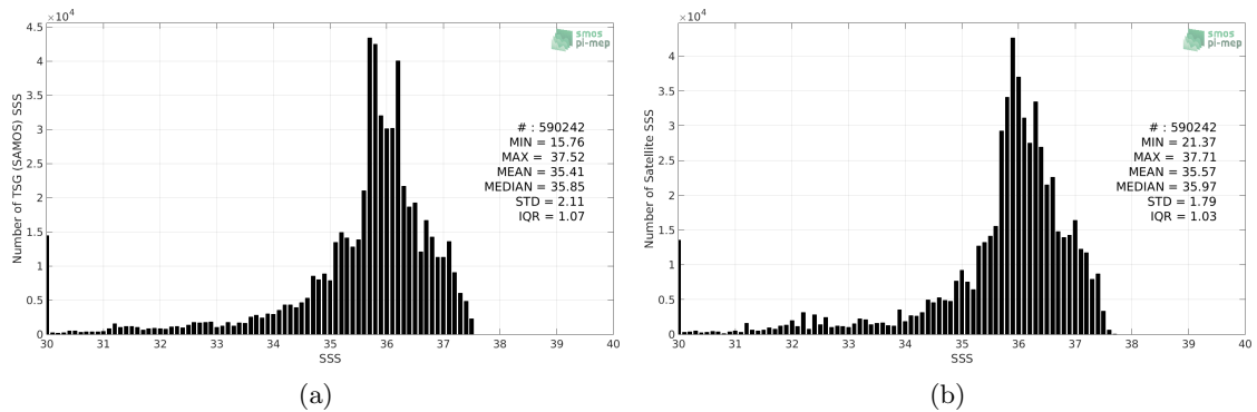
Figure 2: Histograms of SSS from TSG (SAMOS) (a) and CCI L4 Merged-OI v2.31 - 7-day running (ESA) (b) considering all match-up pairs per bins of 0.1 over the Tropical Atlantic Ocean Pi-MEP region and for the full satellite product period.
