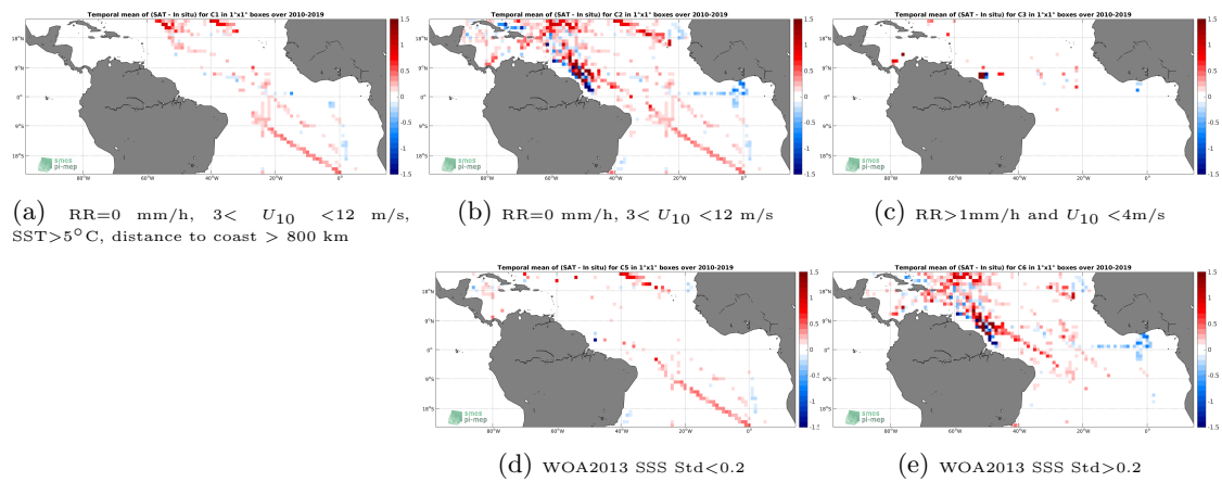
Figure 12: Temporal mean gridded over spatial boxes of size 1^\circ \times 1^\circ of \Delta SSS (CCI L4 Merged-OI v2.31 - 7-day running (ESA) - TSG (SAMOS)) for 5 different subdatasets corresponding to:RR=0 mm/h, 3 < U_{10} < 12 m/s, SST >5^\circ C, distance to coast > 800 km (a), RR=0 mm/h, 3 < U_{10} < 12 m/s (b), RR >1 mm/h and U_{10} < 4 m/s (c), WOA2013 SSS Std <0.2 (d), WOA2013 SSS Std >0.2 (e).
