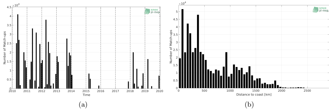
Figure 1: Number of match-ups between TSG (SAMOS) and CCI L4 Merged-OI v2.31 - 7-day running (ESA) SSS as a function of time (a) and as function of the distance to coast (b) over the Tropical Atlantic Ocean Pi-MEP region and for the full satellite product period.
