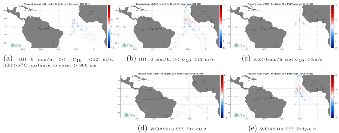
Figure 12: Temporal mean gridded over spatial boxes of size 1^\circ \times 1^\circ of \Delta SSS (CCI SSS L4 Merged-OI v2.31 - 7-day running (ESA) - TSG (Polarstern)) for 5 different subdatasets corresponding to:RR=0 mm/h, 3 < U_{10} < 12 m/s, SST>5°C, distance to coast > 800 km (a), RR=0 mm/h, 3 < U_{10} < 12 m/s (b), RR>1mm/h and U_{10} < 4 m/s (c), WOA2013 SSS Std<0.2 (d), WOA2013 SSS Std>0.2 (e).
