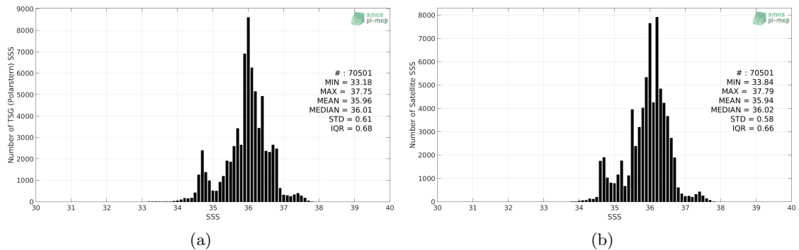
Figure 2: Histograms of SSS from TSG (Polarstern) (a) and CCI SSS L4 Merged-OI v2.31 - 7-day running (ESA) (b) considering all match-up pairs per bins of 0.1 over the Tropical Atlantic Ocean Pi-MEP region and for the full satellite product period.
