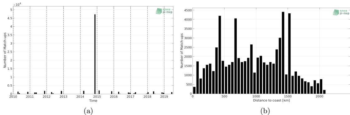
Figure 1: Number of match-ups between TSG (Polarstern) and CCI SSS L4 Merged-OI v2.31 - 7-day running (ESA) SSS as a function of time (a) and as function of the distance to coast (b) over the Tropical Atlantic Ocean Pi-MEP region and for the full satellite product period.
