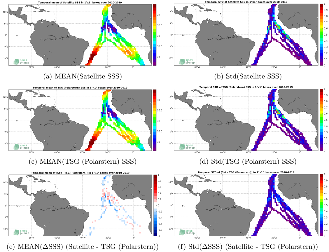
Figure 6: Temporal mean (left) and Std (right) of SSS from CCI SSS L4 Merged-OI v2.31 - 7-day running (ESA) (top), TSG (Polarstern) (middle), and of \Delta SSS (Satellite - TSG (Polarstern)). Only match-up pairs are used to generate these maps.
