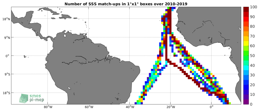
Figure 4: Number of SSS match-ups between TSG (Polarstern) SSS and the CCI SSS L4 Merged-OI v2.31 - 7-day running (ESA) SSS product for the Tropical Atlantic Ocean Pi-MEP region over 1^\circ \times 1^\circ boxes and for the full satellite product period.
