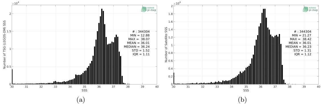
Figure 2: Histograms of SSS from TSG (LEGOS-DM) (a) and CCI L4 Merged-OI v2.31 - 7-day running (ESA) (b) considering all match-up pairs per bins of 0.1 over the Tropical Atlantic Ocean Pi-MEP region and for the full satellite product period.
