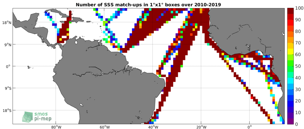
Figure 4: Number of SSS match-ups between TSG (LEGOS-DM) SSS and the CCI L4 Merged-OI v2.31 - 7-day running (ESA) SSS product for the Tropical Atlantic Ocean Pi-MEP region over 1°x1° boxes and for the full satellite product period.
