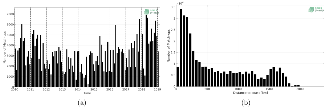
Figure 1: Number of match-ups between TSG (LEGOS-DM) and CCI L4 Merged-OI v2.31 - 7-day running (ESA) SSS as a function of time (a) and as function of the distance to coast (b) over the Tropical Atlantic Ocean Pi-MEP region and for the full satellite product period.
