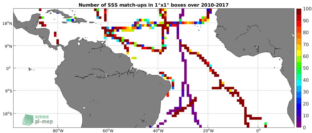
Figure 4: Number of SSS match-ups between TSG (GOSUD-Sailing-ship) SSS and the CCI SSS L4 Merged-OI v2.31 - 7-day running (ESA) SSS product for the Tropical Atlantic Ocean Pi-MEP region over 1^\circ \times 1^\circ boxes and for the full satellite product period.
