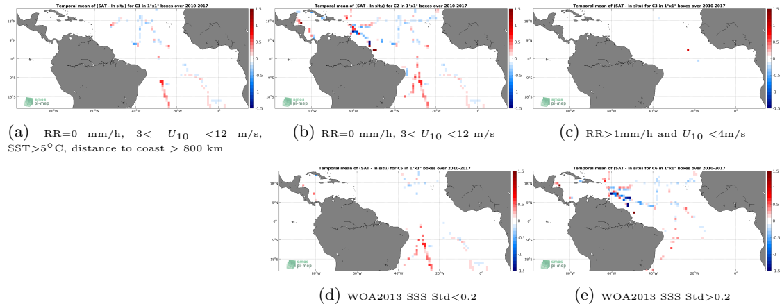
Figure 12: Temporal mean gridded over spatial boxes of size 1^{\circ}\times 1^{\circ} of \Delta SSS (CCI SSS L4 Merged-OI v2.31 - 7-day running (ESA) - TSG (GOSUD-Sailing-ship)) for 5 different subdatasets corresponding to:RR=0 mm/h, 3 < U_{10} < 12 m/s, SST >5^{\circ}\text{C} , distance to coast > 800 km (a), RR=0 mm/h, 3 < U_{10} < 12 m/s (b), RR >1 mm/h and U_{10} < 4 m/s (c), WOA2013 SSS Std <0.2 (d), WOA2013 SSS Std >0.2 (e).
