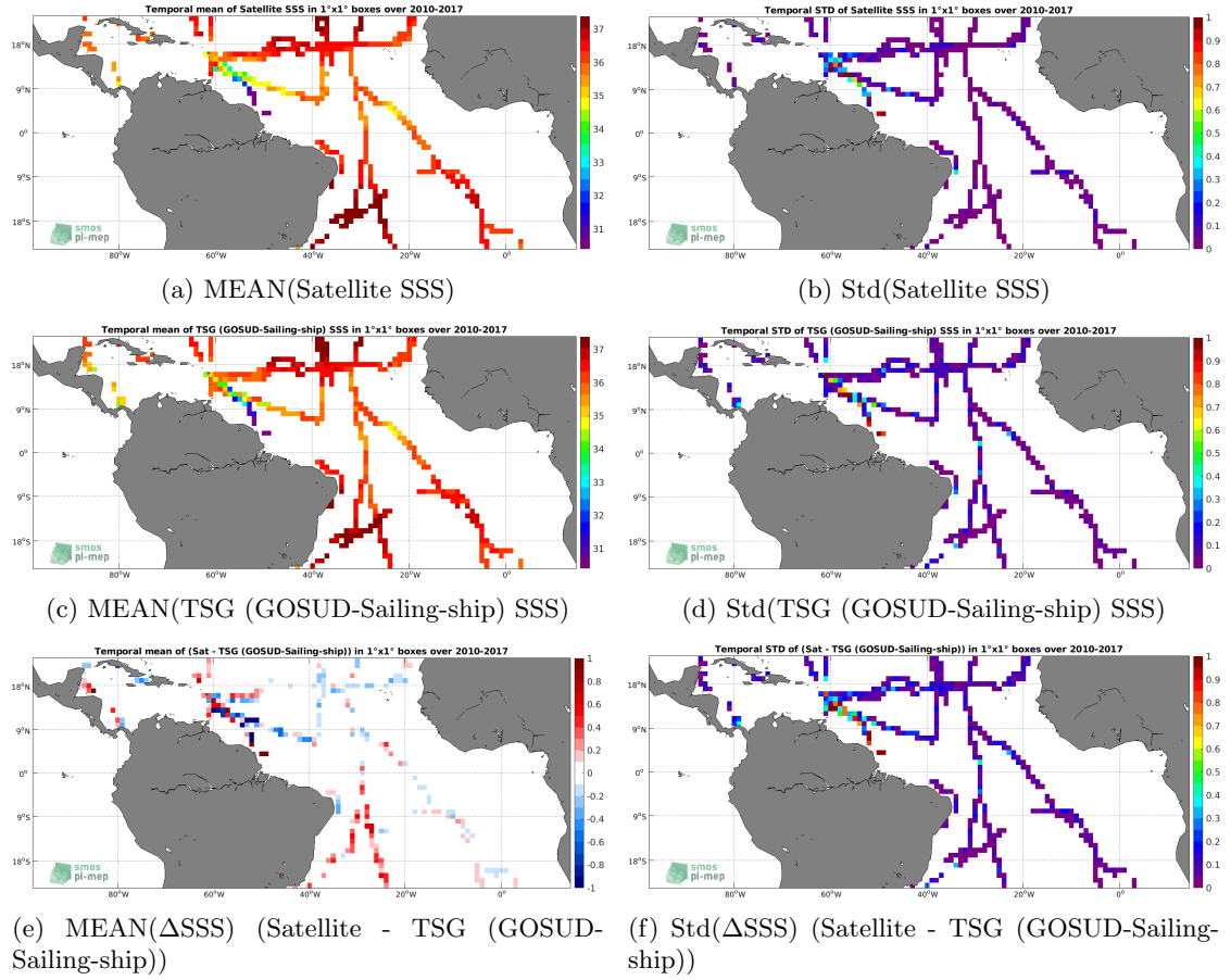
Figure 6: Temporal mean (left) and Std (right) of SSS from CCI SSS L4 Merged-OI v2.31 - 7-day running (ESA) (top), TSG (GOSUD-Sailing-ship) (middle), and of \Delta SSS (Satellite - TSG (GOSUD-Sailing-ship)). Only match-up pairs are used to generate these maps.
