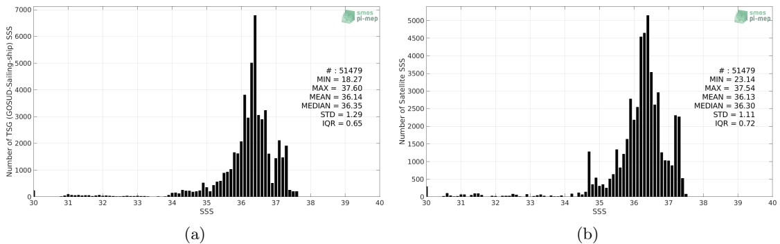
Figure 2: Histograms of SSS from TSG (GOSUD-Sailing-ship) (a) and CCI SSS L4 Merged-OI v2.31 - 7-day running (ESA) (b) considering all match-up pairs per bins of 0.1 over the Tropical Atlantic Ocean Pi-MEP region and for the full satellite product period.
