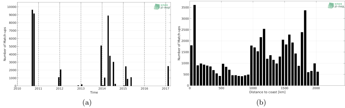
Figure 1: Number of match-ups between TSG (GOSUD-Sailing-ship) and CCI L4 Merged-OI v2.31 - 7-day running (ESA) SSS as a function of time (a) and as function of the distance to coast (b) over the Tropical Atlantic Ocean Pi-MEP region and for the full satellite product period.
