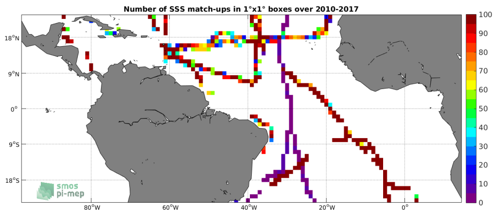
Figure 4: Number of SSS match-ups between TSG (GOSUD-Sailing-ship) SSS and the CCI L4 Merged-OI v2.31 - 7-day running (ESA) SSS product for the Tropical Atlantic Ocean Pi-MEP region over 1^\circ \times 1^\circ boxes and for the full satellite product period.
