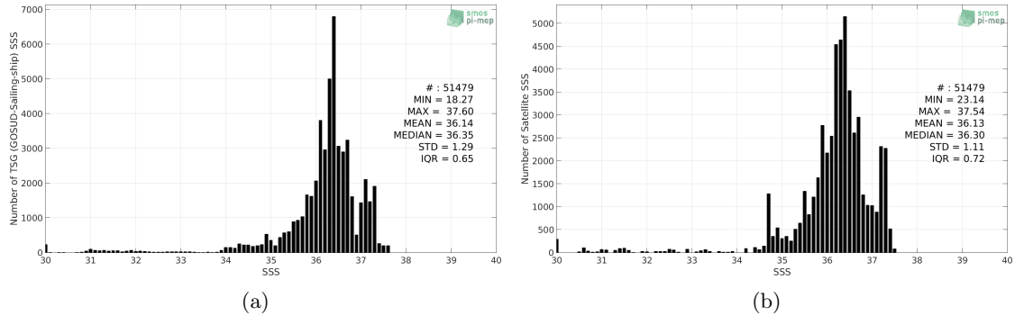
Figure 2: Histograms of SSS from TSG (GOSUD-Sailing-ship) (a) and CCI L4 Merged-OI v2.31 - 7-day running (ESA) (b) considering all match-up pairs per bins of 0.1 over the Tropical Atlantic Ocean Pi-MEP region and for the full satellite product period.
