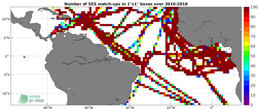
Figure 4: Number of SSS match-ups between TSG (GOSUD-Research-vessel) SSS and the CCI SSS L4 Merged-OI v2.31 - 7-day running (ESA) SSS product for the Tropical Atlantic Ocean Pi-MEP region over 1^\circ \times 1^\circ boxes and for the full satellite product period.
