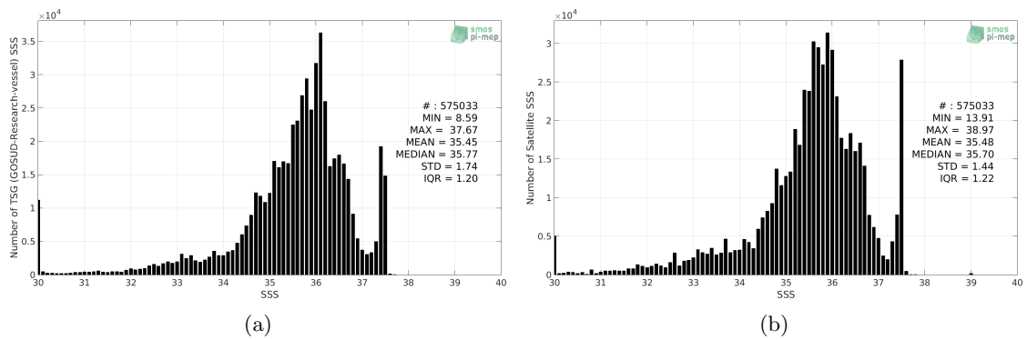
Figure 2: Histograms of SSS from TSG (GOSUD-Research-vessel) (a) and CCI SSS L4 Merged-OI v2.31 - 7-day running (ESA) (b) considering all match-up pairs per bins of 0.1 over the Tropical Atlantic Ocean Pi-MEP region and for the full satellite product period.
