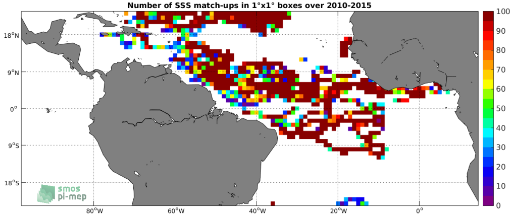
Figure 3: Number of SSS match-ups between Surface drifters SSS and the CCI SSS L4 Merged-OI v2.31 - 7-day running (ESA) SSS product for the Tropical Atlantic Ocean Pi-MEP region over 1°x1° boxes and for the full satellite product period.
