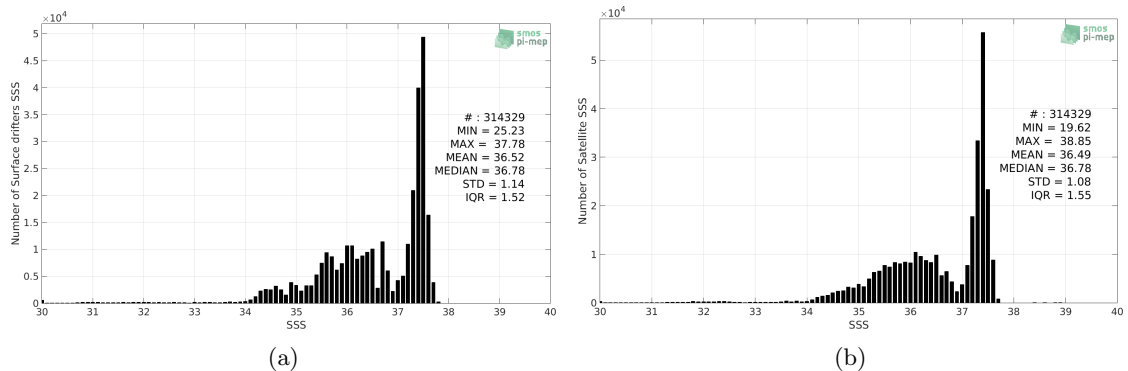
Figure 2: Histograms of SSS from Surface drifters (a) and CCI SSS L4 Merged-OI v2.31 - 7-day running (ESA) (b) considering all match-up pairs per bins of 0.1 over the Tropical Atlantic Ocean Pi-MEP region and for the full satellite product period.
