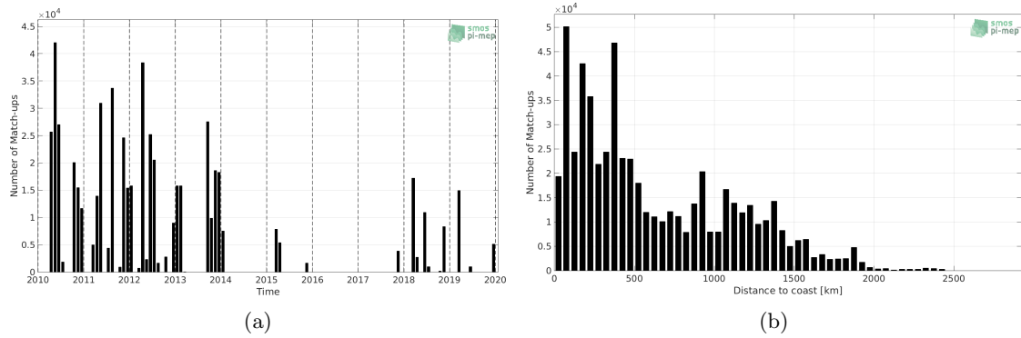
Figure 1: Number of match-ups between TSG (SAMOS) and CCI L4 Merged-OI v2.31 - 30-day running (ESA) SSS as a function of time (a) and as function of the distance to coast (b) over the Tropical Atlantic Ocean Pi-MEP region and for the full satellite product period.
