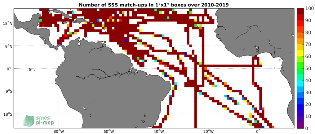
Figure 4: Number of SSS match-ups between TSG (SAMOS) SSS and the CCI L4 Merged-OI v2.31 - 30-day running (ESA) SSS product for the Tropical Atlantic Ocean Pi-MEP region over 1°x1° boxes and for the full satellite product period.
