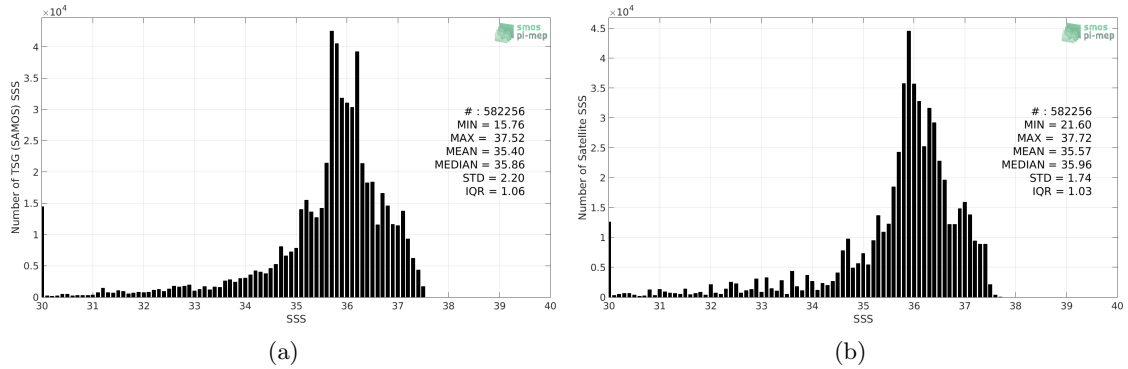
Figure 2: Histograms of SSS from TSG (SAMOS) (a) and CCI L4 Merged-OI v2.31 - 30-day running (ESA) (b) considering all match-up pairs per bins of 0.1 over the Tropical Atlantic Ocean Pi-MEP region and for the full satellite product period.
