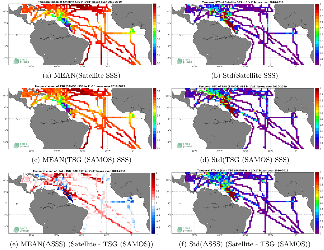
Figure 6: Temporal mean (left) and Std (right) of SSS from CCI L4 Merged-OI v2.31 - 30-day running (ESA) (top), TSG (SAMOS) (middle), and of \Delta SSS (Satellite - TSG (SAMOS)). Only match-up pairs are used to generate these maps.
