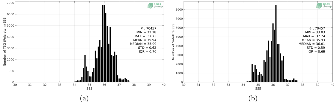
Figure 2: Histograms of SSS from TSG (Polarstern) (a) and CCI SSS L4 Merged-OI v2.31 - 30-day running (ESA) (b) considering all match-up pairs per bins of 0.1 over the Tropical Atlantic Ocean Pi-MEP region and for the full satellite product period.
