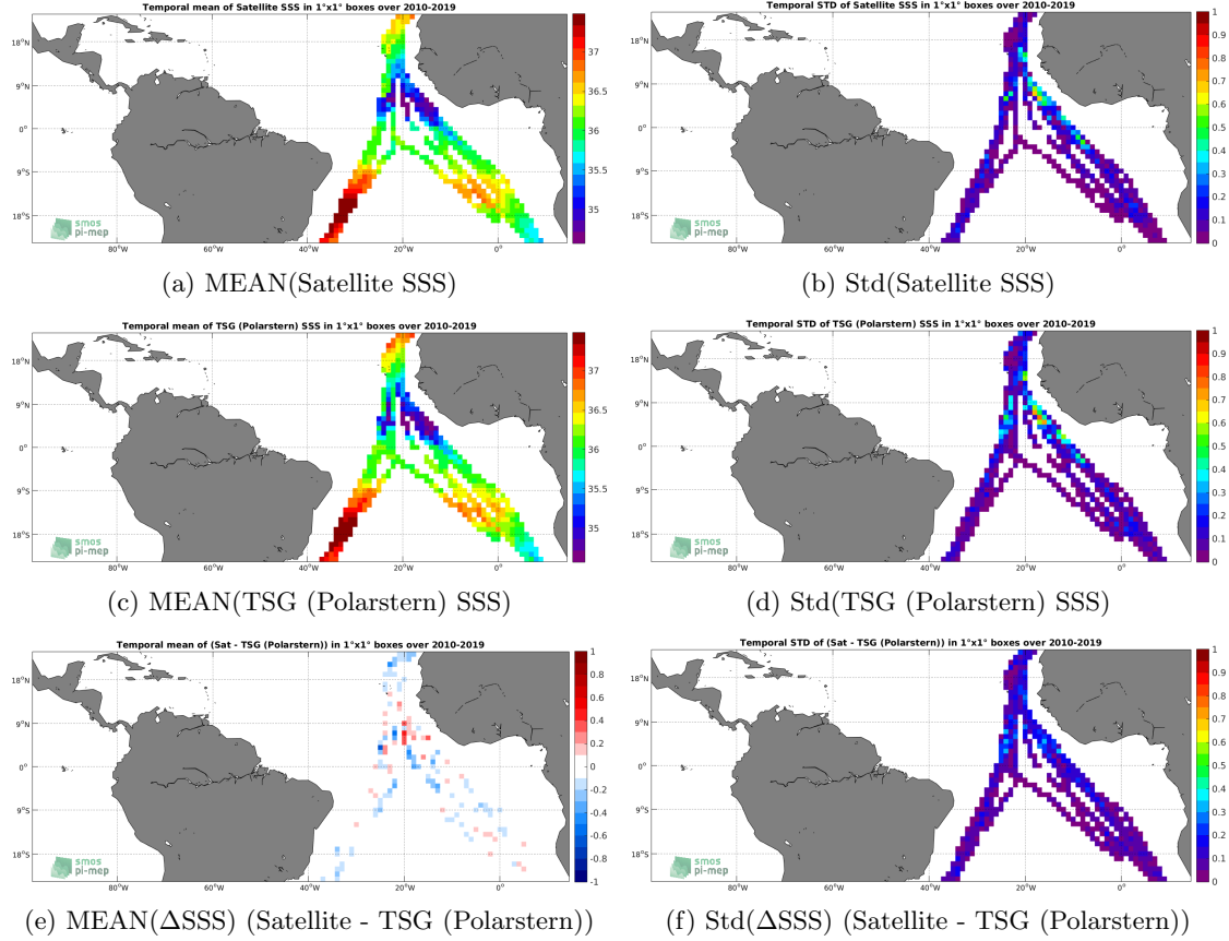
Figure 6: Temporal mean (left) and Std (right) of SSS from CCI SSS L4 Merged-OI v2.31 - 30-day running (ESA) (top), TSG (Polarstern) (middle), and of \Delta SSS (Satellite - TSG (Polarstern)). Only match-up pairs are used to generate these maps.
