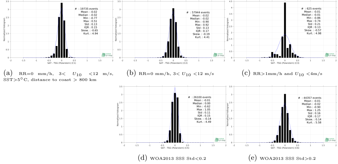
Figure 13: Normalized histogram of \Delta SSS (CCI SSS L4 Merged-OI v2.31 - 30-day running (ESA) - TSG (Polarstern)) for 5 different subdatasets corresponding to: RR=0 mm/h, 3 < U_{10} < 12 m/s, SST>5°C, distance to coast > 800 km (a), RR=0 mm/h, 3 < U_{10} < 12 m/s (b), RR>1mm/h and U_{10} < 4 m/s (c), WOA2013 SSS Std<0.2 (d), WOA2013 SSS Std>0.2 (e).
