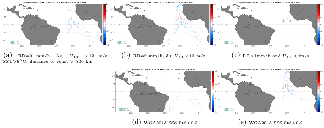
Figure 12: Temporal mean gridded over spatial boxes of size 1^\circ \times 1^\circ of \Delta SSS (CCI SSS L4 Merged-OI v2.31 - 30-day running (ESA) - TSG (Polarstern)) for 5 different subdatasets corresponding to: RR=0 mm/h, 3 < U_{10} < 12 m/s, SST >5^\circ\text{C} , distance to coast > 800 km (a), RR=0 mm/h, 3 < U_{10} < 12 m/s (b), RR >1 mm/h and U_{10} < 4 m/s (c), WOA2013 SSS Std <0.2 (d), WOA2013 SSS Std >0.2 (e).
