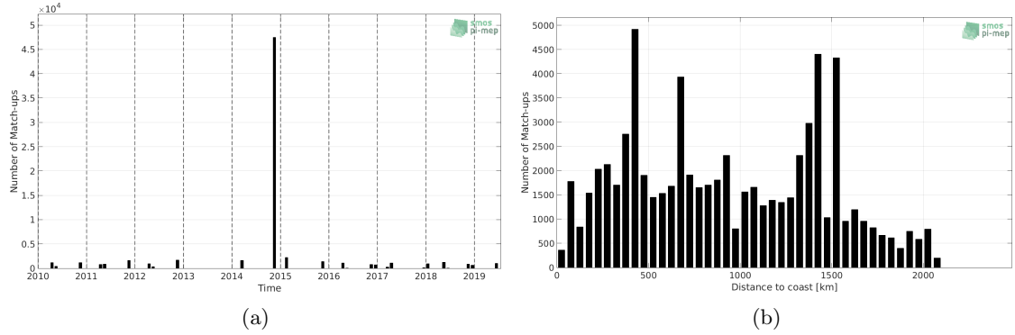
Figure 1: Number of match-ups between TSG (Polarstern) and CCI SSS L4 Merged-OI v2.31 - 30-day running (ESA) SSS as a function of time (a) and as function of the distance to coast (b) over the Tropical Atlantic Ocean Pi-MEP region and for the full satellite product period.
