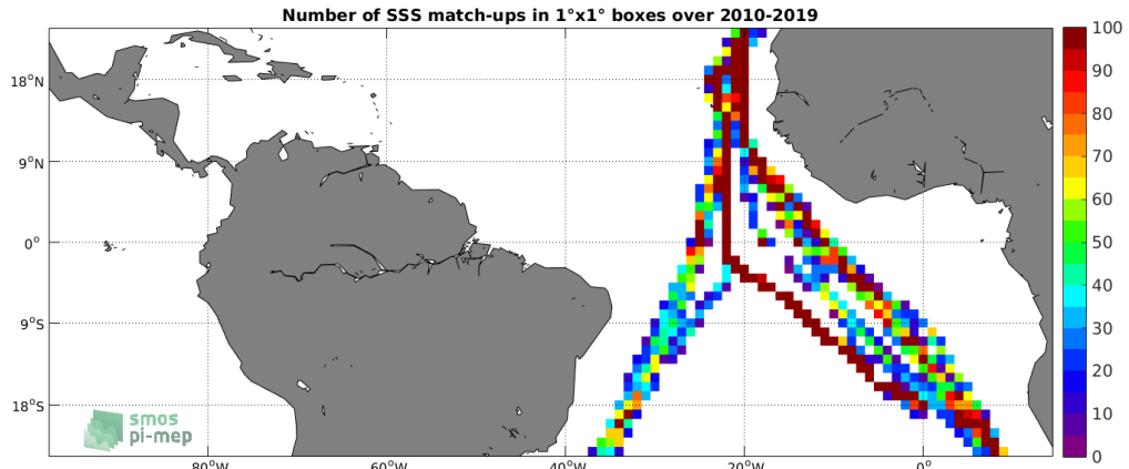
Figure 4: Number of SSS match-ups between TSG (Polarstern) SSS and the CCI SSS L4 Merged-OI v2.31 - 30-day running (ESA) SSS product for the Tropical Atlantic Ocean Pi-MEP region over 1^\circ \times 1^\circ boxes and for the full satellite product period.
