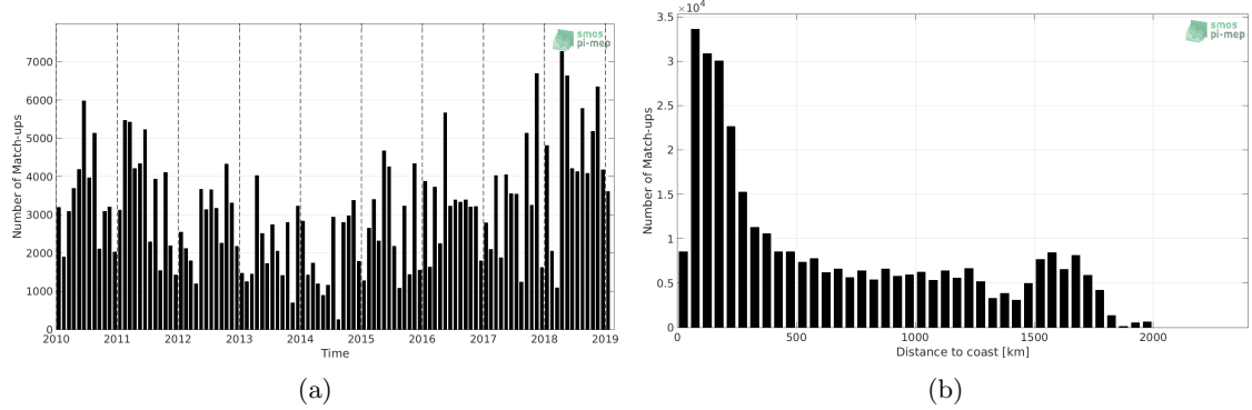
Figure 1: Number of match-ups between TSG (LEGOS-DM) and CCI SSS L4 Merged-OI v2.31 - 30-day running (ESA) SSS as a function of time (a) and as function of the distance to coast (b) over the Tropical Atlantic Ocean Pi-MEP region and for the full satellite product period.
