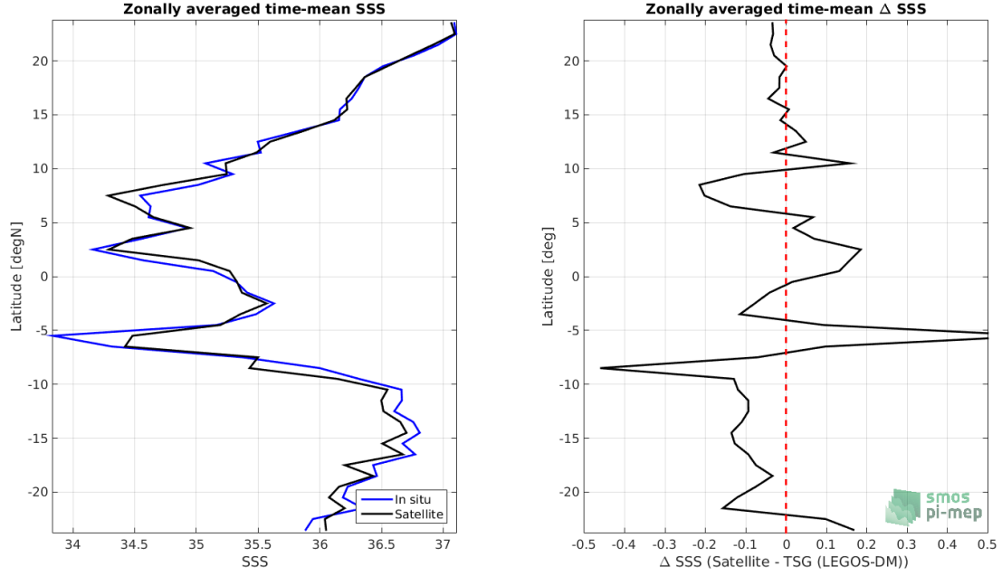
Figure 8: Left panel: Zonal mean SSS from CCI SSS L4 Merged-OI v2.31 - 30-day running (ESA) satellite product (black) and from TSG (LEGOS-DM) (blue). Right panel: Zonal mean of \Delta\text{SSS} (Satellite - TSG (LEGOS-DM)) for all the collected Pi-MEP match-up pairs estimated over the full satellite product period.
