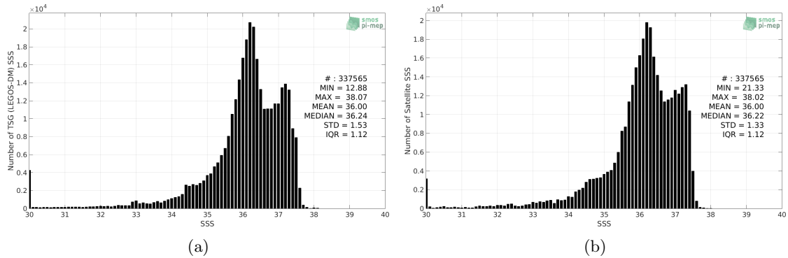
Figure 2: Histograms of SSS from TSG (LEGOS-DM) (a) and CCI SSS L4 Merged-OI v2.31 - 30-day running (ESA) (b) considering all match-up pairs per bins of 0.1 over the Tropical Atlantic Ocean Pi-MEP region and for the full satellite product period.
