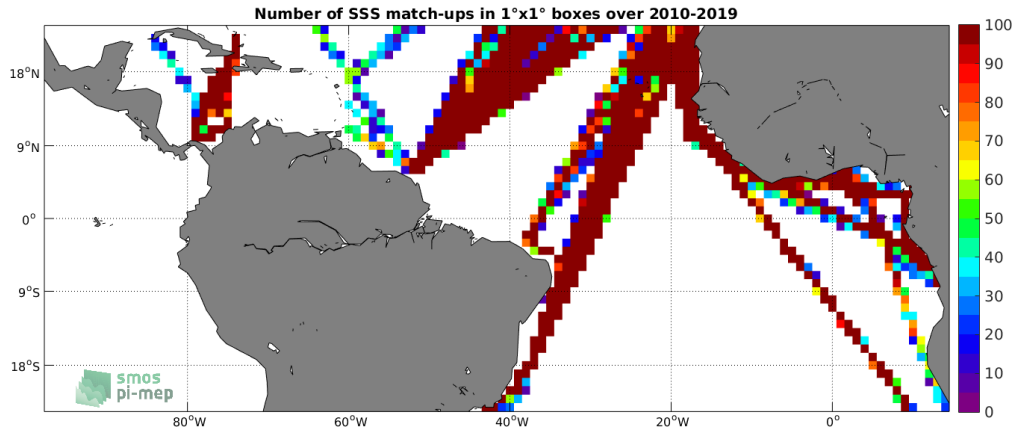
Figure 4: Number of SSS match-ups between TSG (LEGOS-DM) SSS and the CCI SSS L4 Merged-OI v2.31 - 30-day running (ESA) SSS product for the Tropical Atlantic Ocean Pi-MEP region over 1^\circ \times 1^\circ boxes and for the full satellite product period.
