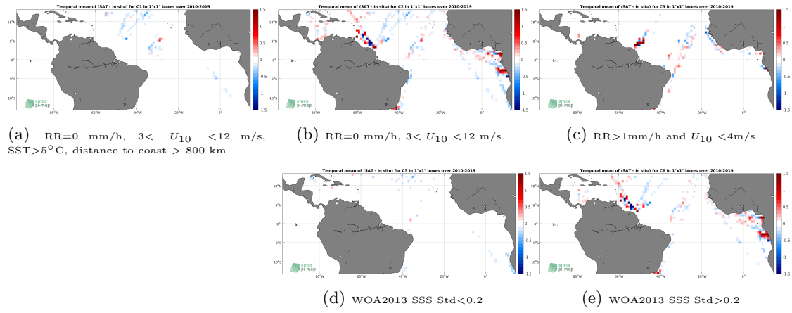
Figure 12: Temporal mean gridded over spatial boxes of size 1^\circ \times 1^\circ of \Delta SSS (CCI L4 Merged-OI v2.31 - 30-day running (ESA) - TSG (LEGOS-DM)) for 5 different subdatasets corresponding to: RR=0 mm/h, 3 < U_{10} < 12 m/s, SST >5^\circ\text{C} , distance to coast > 800 km (a), RR=0 mm/h, 3 < U_{10} < 12 m/s (b), RR >1 mm/h and U_{10} < 4 m/s (c), WOA2013 SSS Std <0.2 (d), WOA2013 SSS Std >0.2 (e).
