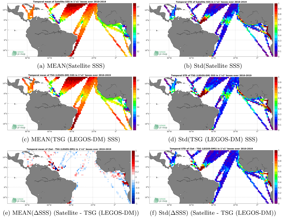
Figure 6: Temporal mean (left) and Std (right) of SSS from CCI L4 Merged-OI v2.31 - 30-day running (ESA) (top), TSG (LEGOS-DM) (middle), and of \Delta SSS (Satellite - TSG (LEGOS-DM)). Only match-up pairs are used to generate these maps.
