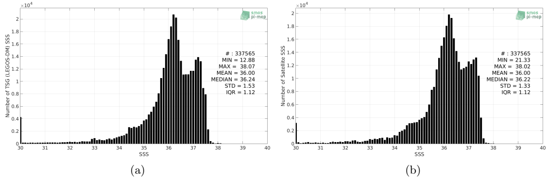
Figure 2: Histograms of SSS from TSG (LEGOS-DM) (a) and CCI L4 Merged-OI v2.31 - 30-day running (ESA) (b) considering all match-up pairs per bins of 0.1 over the Tropical Atlantic Ocean Pi-MEP region and for the full satellite product period.
