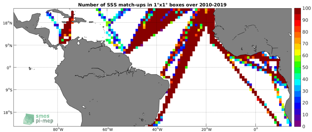
Figure 4: Number of SSS match-ups between TSG (LEGOS-DM) SSS and the CCI L4 Merged-OI v2.31 - 30-day running (ESA) SSS product for the Tropical Atlantic Ocean Pi-MEP region over 1^\circ \times 1^\circ boxes and for the full satellite product period.
