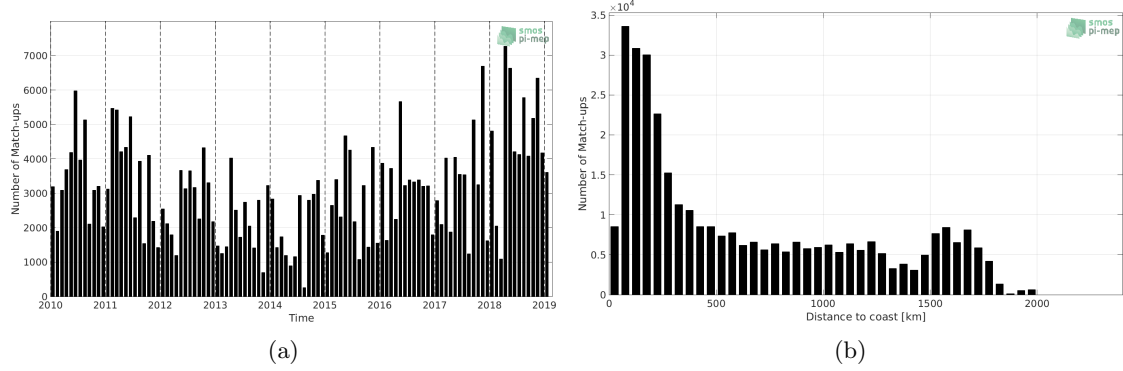
Figure 1: Number of match-ups between TSG (LEGOS-DM) and CCI L4 Merged-OI v2.31 - 30-day running (ESA) SSS as a function of time (a) and as function of the distance to coast (b) over the Tropical Atlantic Ocean Pi-MEP region and for the full satellite product period.
