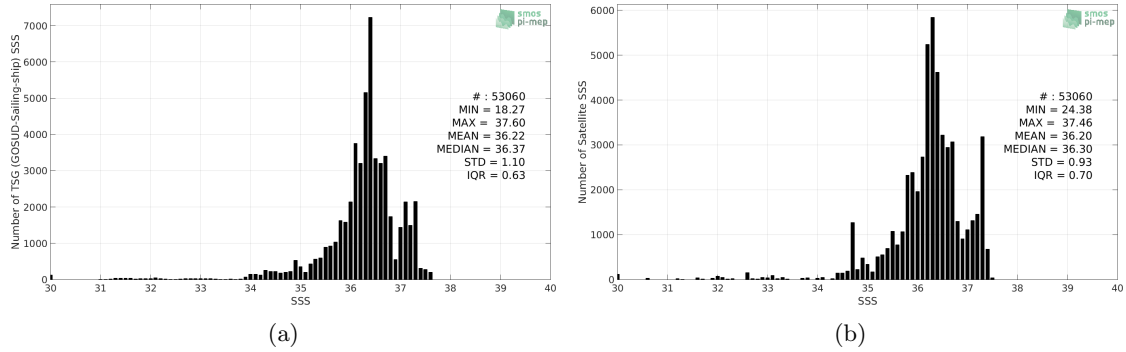
Figure 2: Histograms of SSS from TSG (GOSUD-Sailing-ship) (a) and CCI SSS L4 Merged-OI v2.31 - 30-day running (ESA) (b) considering all match-up pairs per bins of 0.1 over the Tropical Atlantic Ocean Pi-MEP region and for the full satellite product period.
