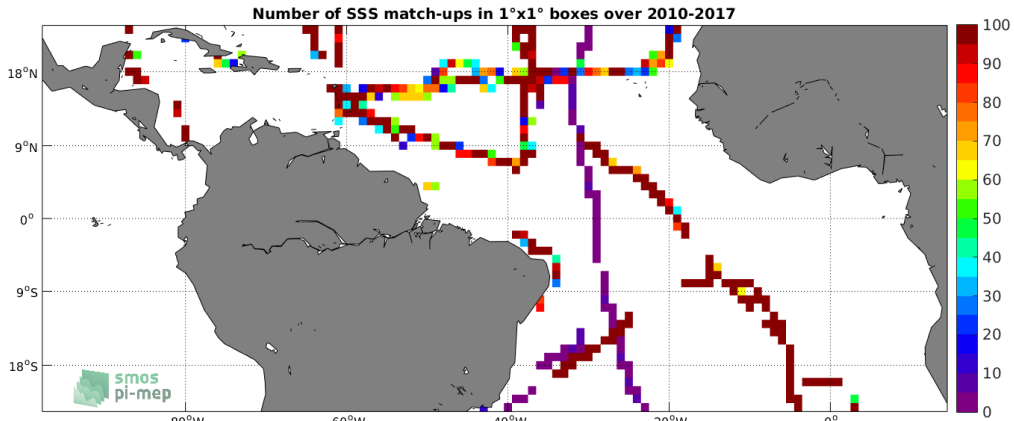
Figure 4: Number of SSS match-ups between TSG (GOSUD-Sailing-ship) SSS and the CCI SSS L4 Merged-OI v2.31 - 30-day running (ESA) SSS product for the Tropical Atlantic Ocean Pi-MEP region over 1^\circ \times 1^\circ boxes and for the full satellite product period.
