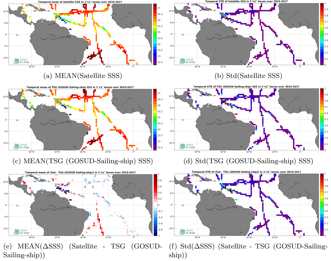
Figure 6: Temporal mean (left) and Std (right) of SSS from CCI SSS L4 Merged-OI v2.31 - 30-day running (ESA) (top), TSG (GOSUD-Sailing-ship) (middle), and of \Delta SSS (Satellite - TSG (GOSUD-Sailing-ship)). Only match-up pairs are used to generate these maps.
