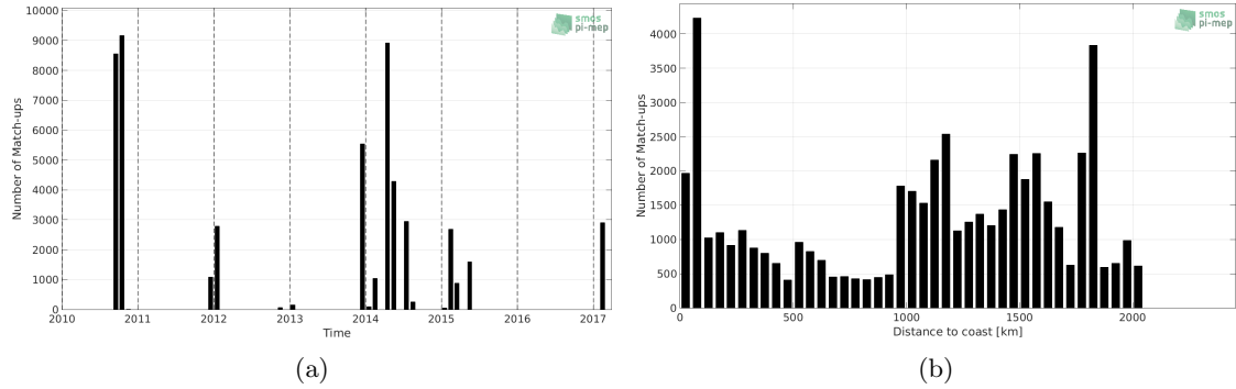
Figure 1: Number of match-ups between TSG (GOSUD-Sailing-ship) and CCI L4 Merged-OI v2.31 - 30-day running (ESA) SSS as a function of time (a) and as function of the distance to coast (b) over the Tropical Atlantic Ocean Pi-MEP region and for the full satellite product period.
