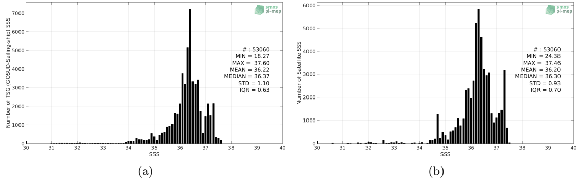
Figure 2: Histograms of SSS from TSG (GOSUD-Sailing-ship) (a) and CCI L4 Merged-OI v2.31 - 30-day running (ESA) (b) considering all match-up pairs per bins of 0.1 over the Tropical Atlantic Ocean Pi-MEP region and for the full satellite product period.
