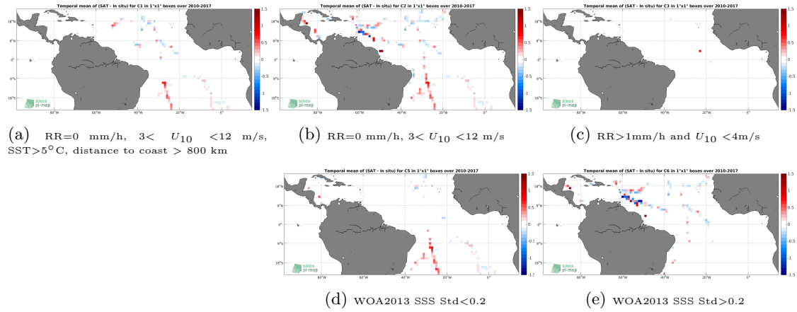
Figure 12: Temporal mean gridded over spatial boxes of size 1^{\circ}\times 1^{\circ} of \Delta SSS (CCI L4 Merged-OI v2.31 - 30-day running (ESA) - TSG (GOSUD-Sailing-ship)) for 5 different subdatasets corresponding to:RR=0 mm/h, 3 < U_{10} < 12 m/s, SST >5^{\circ}\text{C} , distance to coast > 800 km (a), RR=0 mm/h, 3 < U_{10} < 12 m/s (b), RR >1 mm/h and U_{10} < 4 m/s (c), WOA2013 SSS Std <0.2 (d), WOA2013 SSS Std >0.2 (e).
