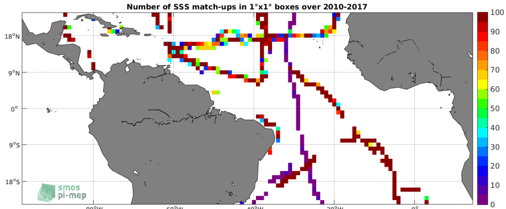
Figure 4: Number of SSS match-ups between TSG (GOSUD-Sailing-ship) SSS and the CCI L4 Merged-OI v2.31 - 30-day running (ESA) SSS product for the Tropical Atlantic Ocean Pi-MEP region over 1^\circ \times 1^\circ boxes and for the full satellite product period.
