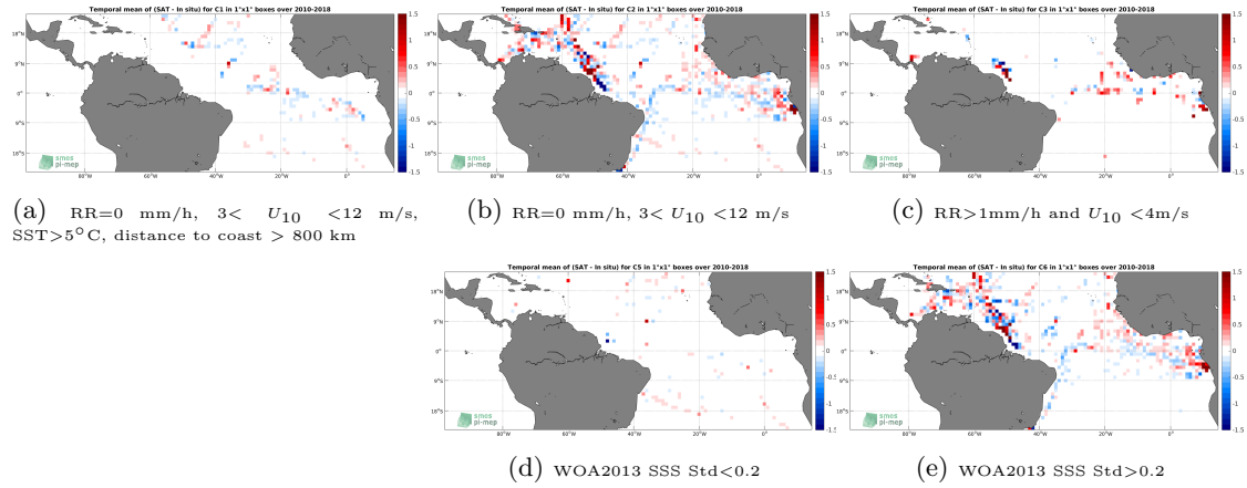
Figure 12: Temporal mean gridded over spatial boxes of size 1^{\circ}\times 1^{\circ} of \Delta SSS (CCI L4 Merged-OI v2.31 - 30-day running (ESA) - TSG (GOSUD-Research-vessel)) for 5 different subdatasets corresponding to:RR=0 mm/h, 3 < U_{10} < 12 m/s, SST >5^{\circ}\text{C} , distance to coast > 800 km (a), RR=0 mm/h, 3 < U_{10} < 12 m/s (b), RR >1 mm/h and U_{10} < 4 m/s (c), WOA2013 SSS Std <0.2 (d), WOA2013 SSS Std >0.2 (e).
