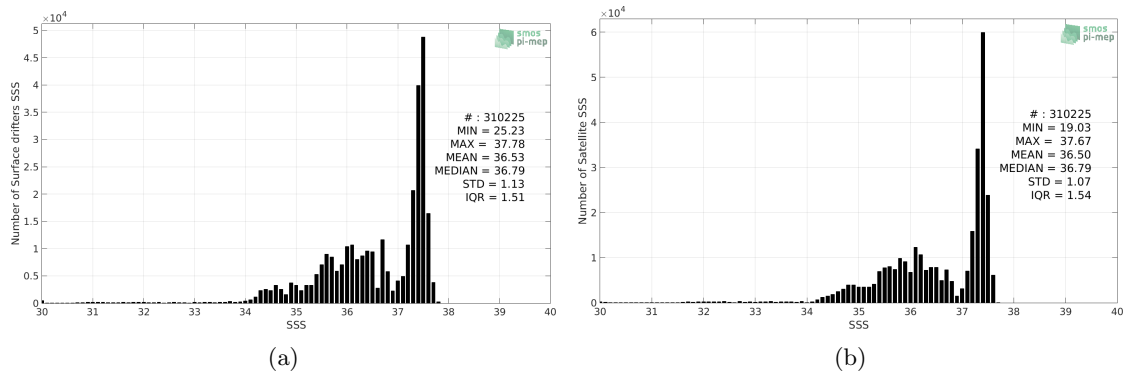
Figure 2: Histograms of SSS from Surface drifters (a) and CCI SSS L4 Merged-OI v2.31 - 30-day running (ESA) (b) considering all match-up pairs per bins of 0.1 over the Tropical Atlantic Ocean Pi-MEP region and for the full satellite product period.
