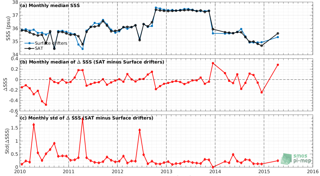
Figure 6: Time series of the monthly median SSS (top), median of \Delta\text{SSS} (Satellite - Surface drifters) and Std of \Delta\text{SSS} (Satellite - Surface drifters) over the Tropical Atlantic Ocean Pi-MEP region considering all match-ups collected by the Pi-MEP.
