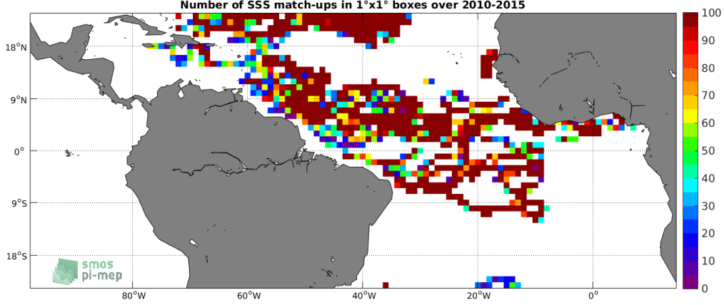
Figure 3: Number of SSS match-ups between Surface drifters SSS and the CCI SSS L4 Merged-OI v2.31 - 30-day running (ESA) SSS product for the Tropical Atlantic Ocean Pi-MEP region over 1^\circ \times 1^\circ boxes and for the full satellite product period.
