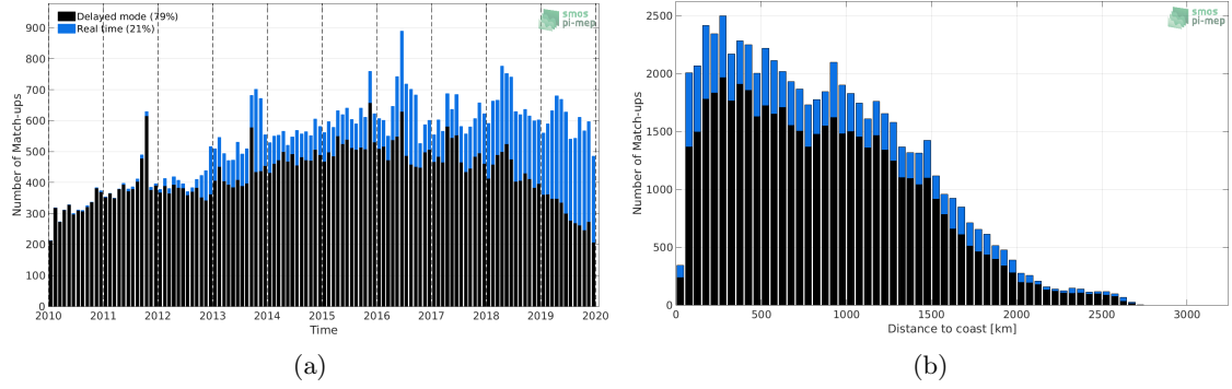
Figure 1: Number of match-ups between Argo and CCI SSS L4 Merged-OI v2.31 - 30-day running (ESA) SSS as a function of time (a) and as function of the distance to coast (b) over the Tropical Atlantic Ocean Pi-MEP region and for the full satellite product period.
