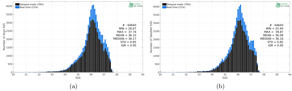
Figure 2: Histograms of SSS from Argo (a) and CCI SSS L4 Merged-OI v2.31 - 30-day running (ESA) (b) considering all match-up pairs per bins of 0.1 over the Tropical Atlantic Ocean Pi-MEP region and for the full satellite product period.
