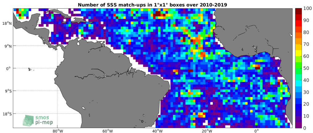
Figure 4: Number of SSS match-ups between Argo SSS and the CCI SSS L4 Merged-OI v2.31 - 30-day running (ESA) SSS product for the Tropical Atlantic Ocean Pi-MEP region over 1^\circ \times 1^\circ boxes and for the full satellite product period.
