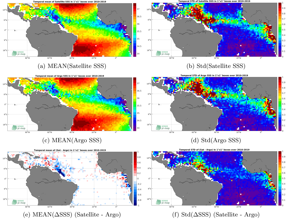
Figure 6: Temporal mean (left) and Std (right) of SSS from CCI L4 Merged-OI v2.31 - 30-day running (ESA) (top), Argo (middle), and of \Delta SSS (Satellite - Argo). Only match-up pairs are used to generate these maps.
