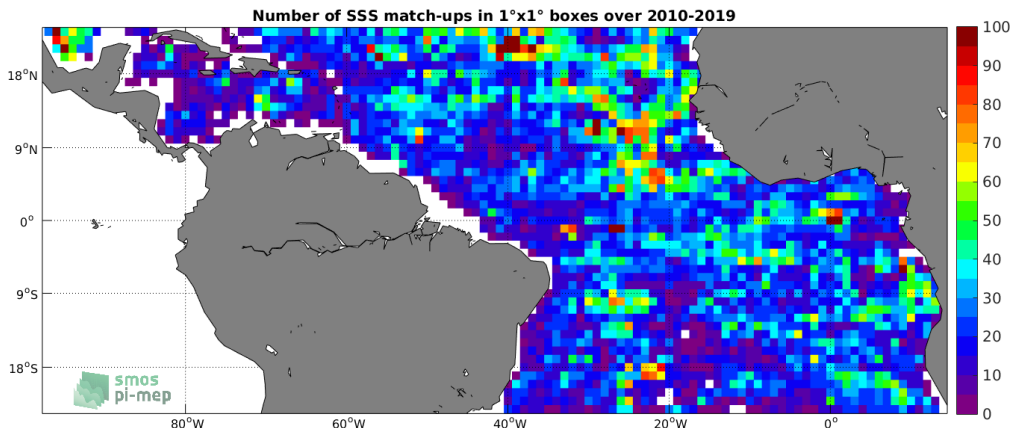
Figure 4: Number of SSS match-ups between Argos SSS and the CCI L4 Merged-OI v2.31 - 30-day running (ESA) SSS product for the Tropical Atlantic Ocean Pi-MEP region over 1°x1° boxes and for the full satellite product period.
