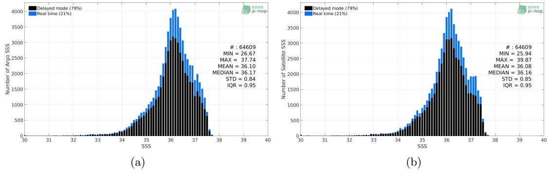
Figure 2: Histograms of SSS from Argo (a) and CCI L4 Merged-OI v2.31 - 30-day running (ESA) (b) considering all match-up pairs per bins of 0.1 over the Tropical Atlantic Ocean Pi-MEP region and for the full satellite product period.
