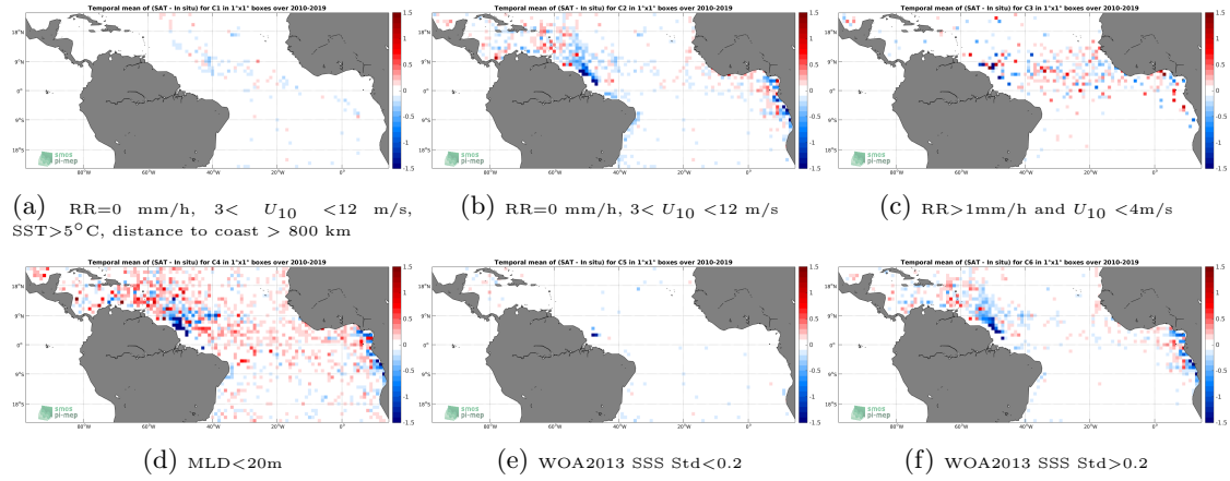
Figure 12: Temporal mean gridded over spatial boxes of size 1^\circ \times 1^\circ of \Delta SSS (CCI L4 Merged-OI v2.31 - 30-day running (ESA) - Argo) for 6 different subdatasets corresponding to: RR=0 mm/h, 3 < U_{10} < 12 m/s, SST > 5^\circ C , distance to coast > 800 km (a), RR=0 mm/h, 3 < U_{10} < 12 m/s (b), RR > 1 mm/h and U_{10} < 4 m/s (c), MLD < 20 m (d), WOA2013 SSS Std < 0.2 (e), WOA2013 SSS Std > 0.2 (f).
