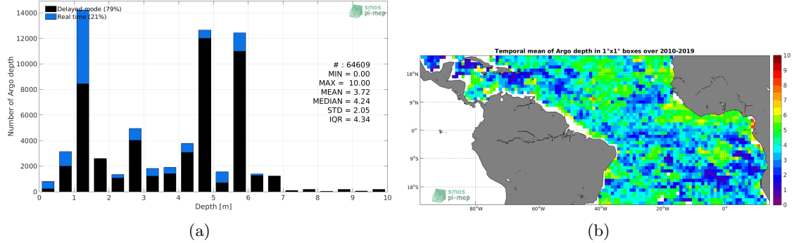
Figure 3: Histograms of the depth of the upper level SSS measurements from Argos in the Match-up DataBase for the Tropical Atlantic Ocean Pi-MEP region (a) and temporal mean spatial distribution of pressure of the in situ SSS data over 1°x1° boxes and for the full satellite product period (b).
