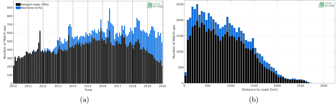
Figure 1: Number of match-ups between Argo and CCI L4 Merged-OI v2.31 - 30-day running (ESA) SSS as a function of time (a) and as function of the distance to coast (b) over the Tropical Atlantic Ocean Pi-MEP region and for the full satellite product period.
