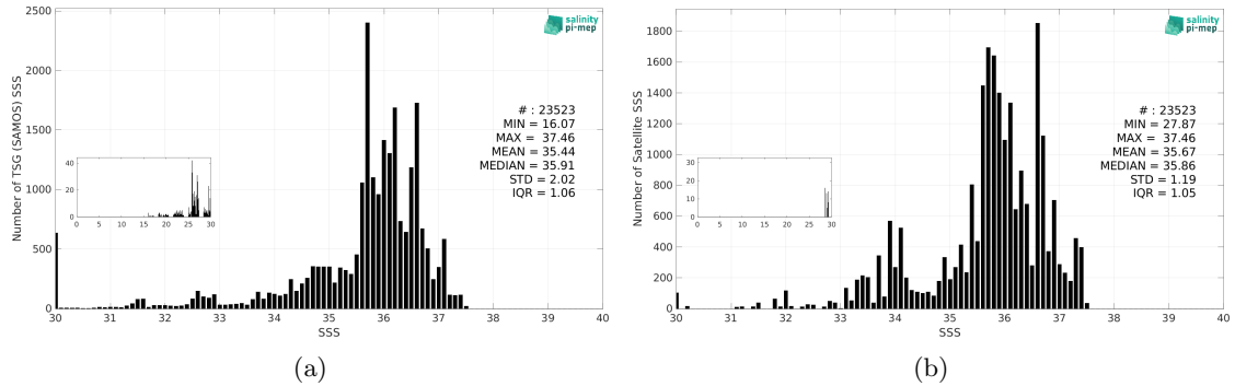
Figure 3: Histograms of SSS from TSG (SAMOS) (a) and Aquarius SSS L4 OI v5 - Weekly (IPRC) (b) considering all match-up pairs per bins of 0.1 over the Tropical Atlantic Ocean Pi-MEP region and for the full satellite product period.
