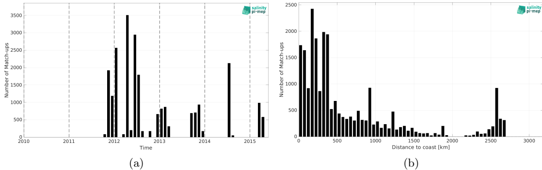
Figure 2: Number of match-ups between TSG (SAMOS) and Aquarius SSS L4 OI v5 - Weekly (IPRC) SSS as a function of time (a) and as function of the distance to coast (b) over the Tropical Atlantic Ocean Pi-MEP region and for the full satellite product period.
