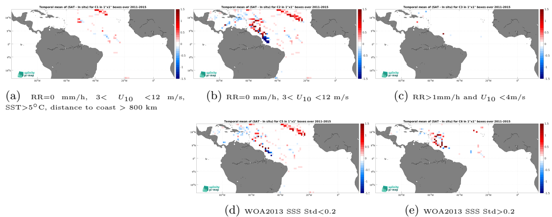
Figure 14: Temporal mean gridded over spatial boxes of size 1^\circ \times 1^\circ of \Delta SSS (Aquarius SSS L4 OI v5 - Weekly (IPRC) - TSG (SAMOS)) for 5 different subdatasets corresponding to:RR=0 mm/h, 3 < U_{10} < 12 m/s, SST >5^\circ\text{C} , distance to coast > 800 km (a), RR=0 mm/h, 3 < U_{10} < 12 m/s (b), RR >1 mm/h and U_{10} < 4 m/s (c), WOA2013 SSS Std <0.2 (d), WOA2013 SSS Std >0.2 (e).
