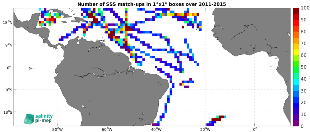
Figure 5: Number of SSS match-ups between TSG (SAMOS) SSS and the Aquarius SSS L4 OI v5 - Weekly (IPRC) SSS product for the Tropical Atlantic Ocean Pi-MEP region over 1^\circ \times 1^\circ boxes and for the full satellite product period.
