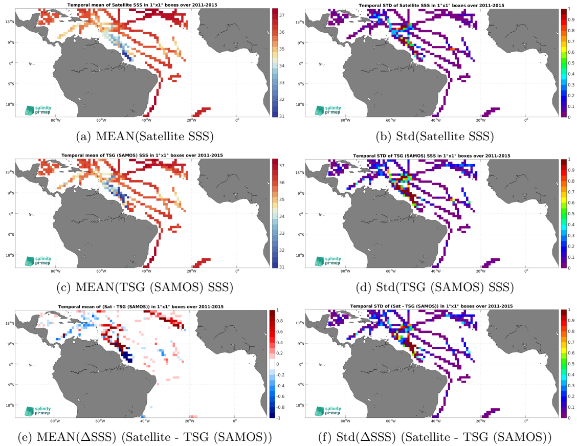
Figure 7: Temporal mean (left) and Std (right) of SSS from Aquarius SSS L4 OI v5 - Weekly (IPRC) (top), TSG (SAMOS) (middle), and of \Delta\text{SSS} (Satellite - TSG (SAMOS)). Only match-up pairs are used to generate these maps.
