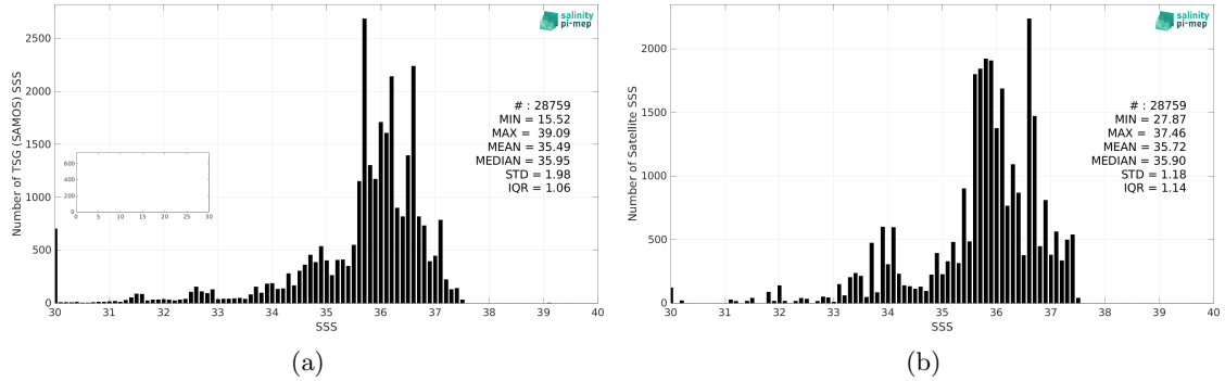
Figure 2: Histograms of SSS from TSG (SAMOS) (a) and Aquarius SSS L4 OI v5 - Weekly (IPRC) (b) considering all match-up pairs per bins of 0.1 over the Tropical Atlantic Ocean Pi-MEP region and for the full satellite product period.
