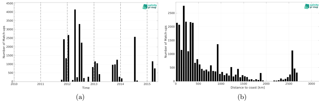
Figure 1: Number of match-ups between TSG (SAMOS) and Aquarius SSS L4 OI v5 - Weekly (IPRC) SSS as a function of time (a) and as function of the distance to coast (b) over the Tropical Atlantic Ocean Pi-MEP region and for the full satellite product period.
