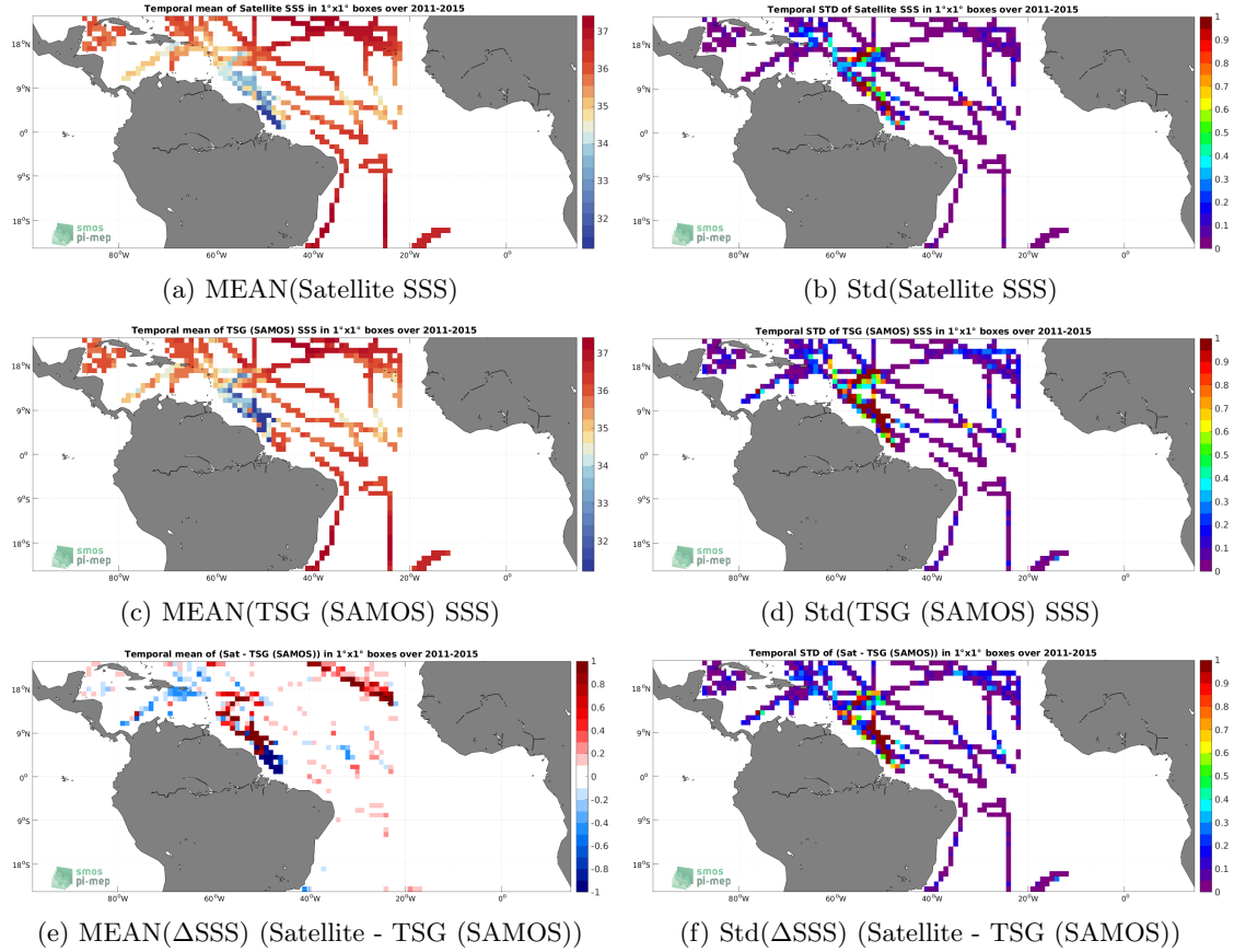
Figure 6: Temporal mean (left) and Std (right) of SSS from Aquarius SSS L4 OI v5 - Weekly (IPRC) (top), TSG (SAMOS) (middle), and of \Delta\text{SSS}(\text{Satellite} - \text{TSG}(\text{SAMOS})) . Only match-up pairs are used to generate these maps.
