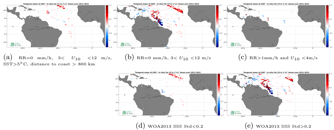
Figure 12: Temporal mean gridded over spatial boxes of size 1°x1° of \Delta SSS (Aquarius SSS L4 OI v5 - Weekly (IPRC) - TSG (SAMOS)) for 5 different subdatasets corresponding to:RR=0 mm/h, 3 < U_{10} < 12 m/s, SST > 5^\circ C , distance to coast > 800 km (a), RR=0 mm/h, 3 < U_{10} < 12 m/s (b), RR>1mm/h and U_{10} < 4 m/s (c), WOA2013 SSS Std<0.2 (d), WOA2013 SSS Std>0.2 (e).
