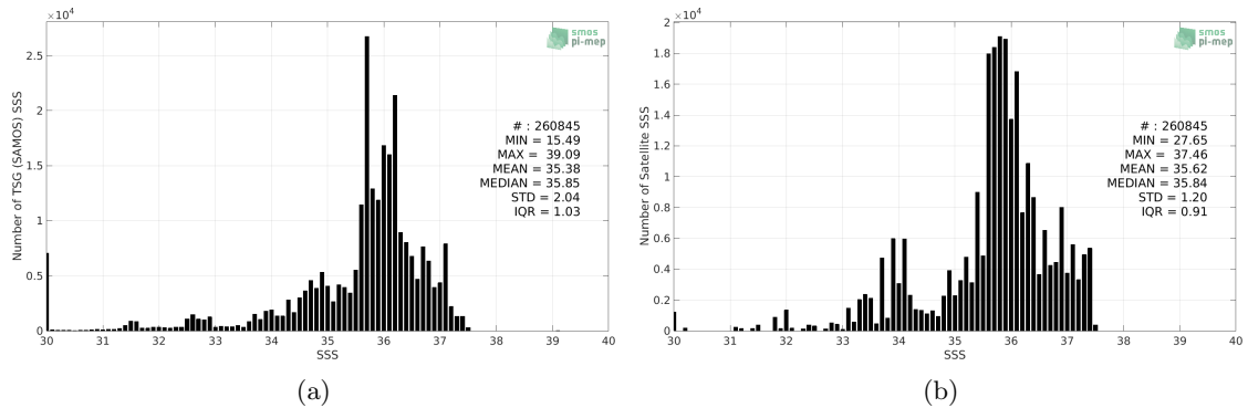
Figure 2: Histograms of SSS from TSG (SAMOS) (a) and Aquarius SSS L4 OI v5 - Weekly (IPRC) (b) considering all match-up pairs per bins of 0.1 over the Tropical Atlantic Ocean Pi-MEP region and for the full satellite product period.
