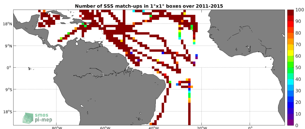
Figure 4: Number of SSS match-ups between TSG (SAMOS) SSS and the Aquarius SSS L4 OI v5 - Weekly (IPRC) SSS product for the Tropical Atlantic Ocean Pi-MEP region over 1^\circ \times 1^\circ boxes and for the full satellite product period.
