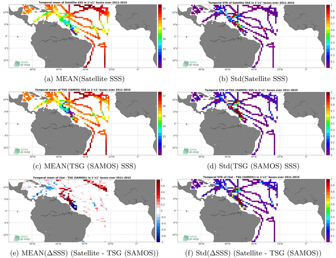
Figure 6: Temporal mean (left) and Std (right) of SSS from Aquarius SSS L4 OI v5 - Weekly (IPRC) (top), TSG (SAMOS) (middle), and of \Delta SSS (Satellite - TSG (SAMOS)). Only match-up pairs are used to generate these maps.
