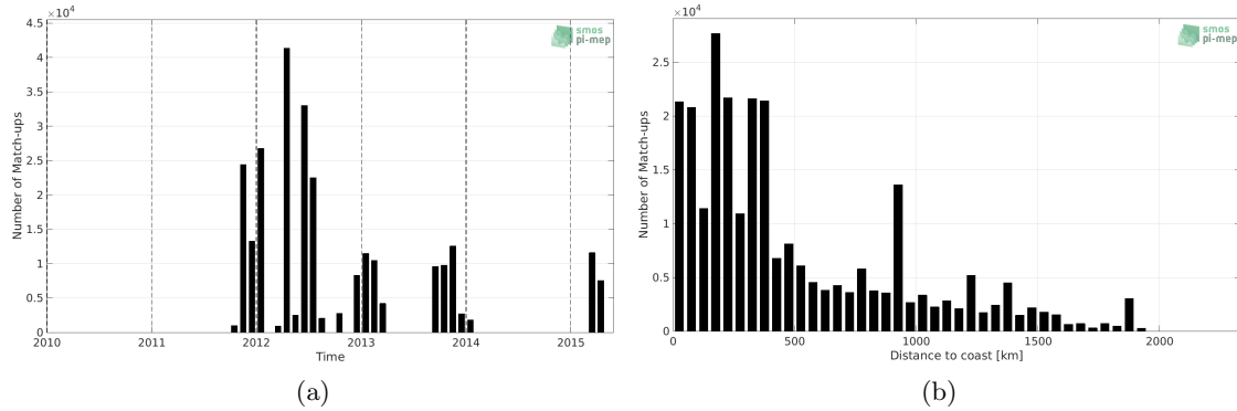
Figure 1: Number of match-ups between TSG (SAMOS) and Aquarius SSS L4 OI v5 - Weekly (IPRC) SSS as a function of time (a) and as function of the distance to coast (b) over the Tropical Atlantic Ocean Pi-MEP region and for the full satellite product period.
