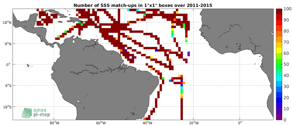
Figure 4: Number of SSS match-ups between TSG-SAMOS SSS and the Aquarius-L4-IPRC-V5-WEEKLY SSS product for the Tropical Atlantic Ocean Pi-MEP region over 1^\circ \times 1^\circ boxes and for the full satellite product period.
