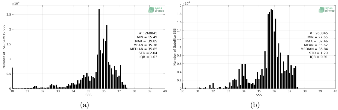
Figure 2: Histograms of SSS from TSG-SAMOS (a) and Aquarius-L4-IPRC-V5-WEEKLY (b) considering all match-up pairs per bins of 0.1 over the Tropical Atlantic Ocean Pi-MEP region and for the full satellite product period.
