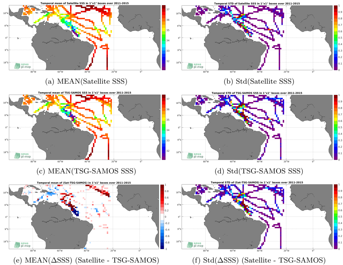
Figure 6: Temporal mean (left) and Std (right) of SSS from Aquarius-L4-IPRC-V5-WEEKLY (top), TSG-SAMOS (middle), and of \Delta SSS (Satellite - TSG-SAMOS). Only match-up pairs are used to generate these maps.
