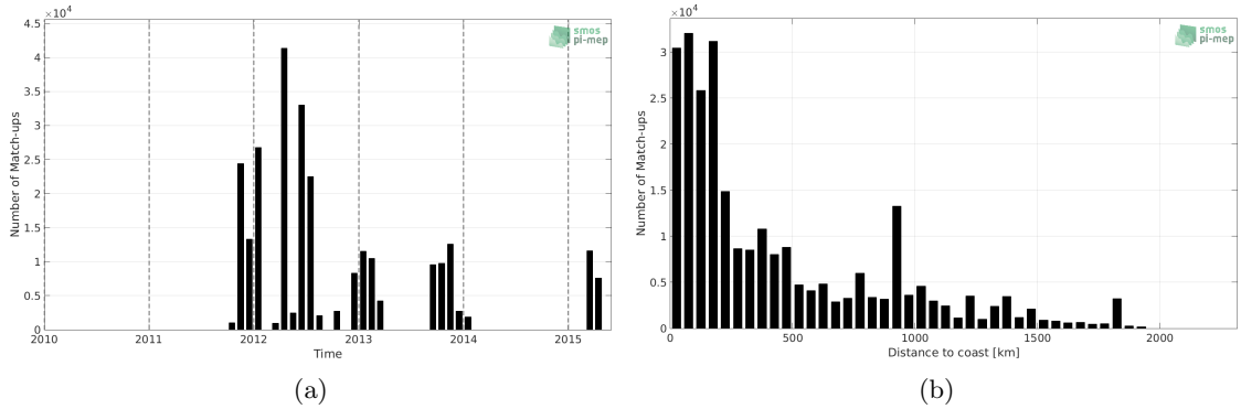
Figure 1: Number of match-ups between TSG-SAMOS and Aquarius-L4-IPRC-V5-WEEKLY SSS as a function of time (a) and as function of the distance to coast (b) over the Tropical Atlantic Ocean Pi-MEP region and for the full satellite product period.
