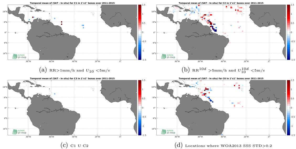
Figure 12: Temporal mean gridded over spatial boxes of size 1^\circ \times 1^\circ of \Delta SSS (Aquarius-L4-IPRC-V5-WEEKLY - TSG-SAMOS) for 4 different subdatasets corresponding to: RR > 1\text{mm/h} and U_{10} < 5\text{m/s} (a), RR^{10d} > 5\text{mm/h} and U_{10}^{10d} < 5\text{m/s} (b), C1 U C2 (c), Locations where WOA2013 SSS STD > 0.2 (d).
