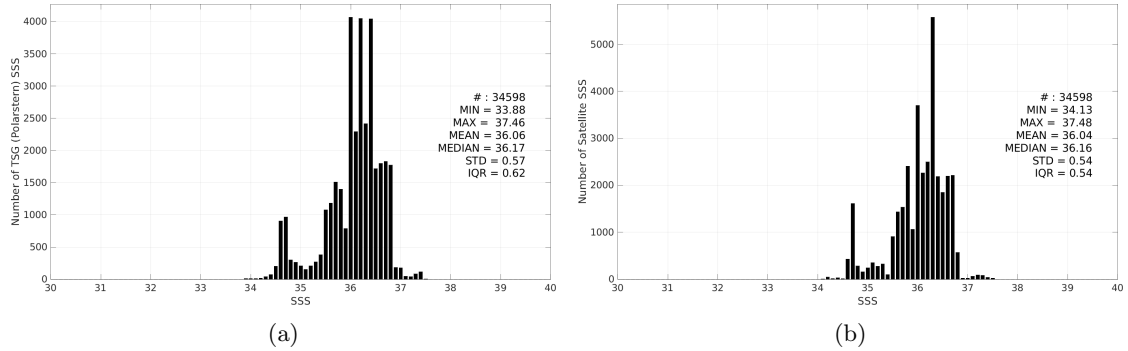
Figure 3: Histograms of SSS from TSG (Polarstern) (a) and Aquarius SSS L4 OI v5 - Weekly (IPRC) (b) considering all match-up pairs per bins of 0.1 over the Tropical Atlantic Ocean Pi-MEP region and for the full satellite product period.
