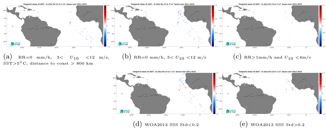
Figure 14: Temporal mean gridded over spatial boxes of size 1^\circ \times 1^\circ of \Delta SSS (Aquarius SSS L4 OI v5 - Weekly (IPRC) - TSG (Polarstern)) for 5 different subdatasets corresponding to:RR=0 mm/h, 3 < U_{10} < 12 m/s, SST >5^\circ\text{C} , distance to coast > 800 km (a), RR=0 mm/h, 3 < U_{10} < 12 m/s (b), RR >1 mm/h and U_{10} < 4 m/s (c), WOA2013 SSS Std <0.2 (d), WOA2013 SSS Std >0.2 (e).
