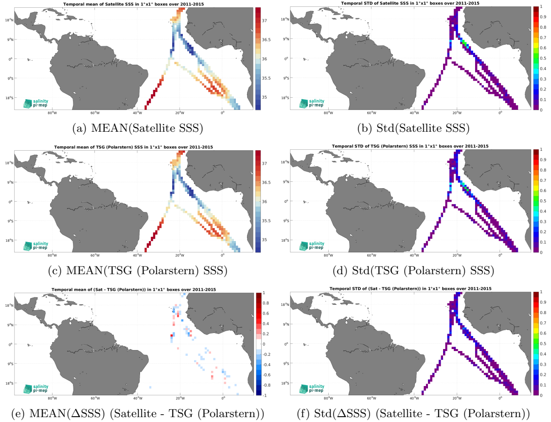
Figure 7: Temporal mean (left) and Std (right) of SSS from Aquarius SSS L4 OI v5 - Weekly (IPRC) (top), TSG (Polarstern) (middle), and of \Delta\text{SSS} (Satellite - TSG (Polarstern)). Only match-up pairs are used to generate these maps.
