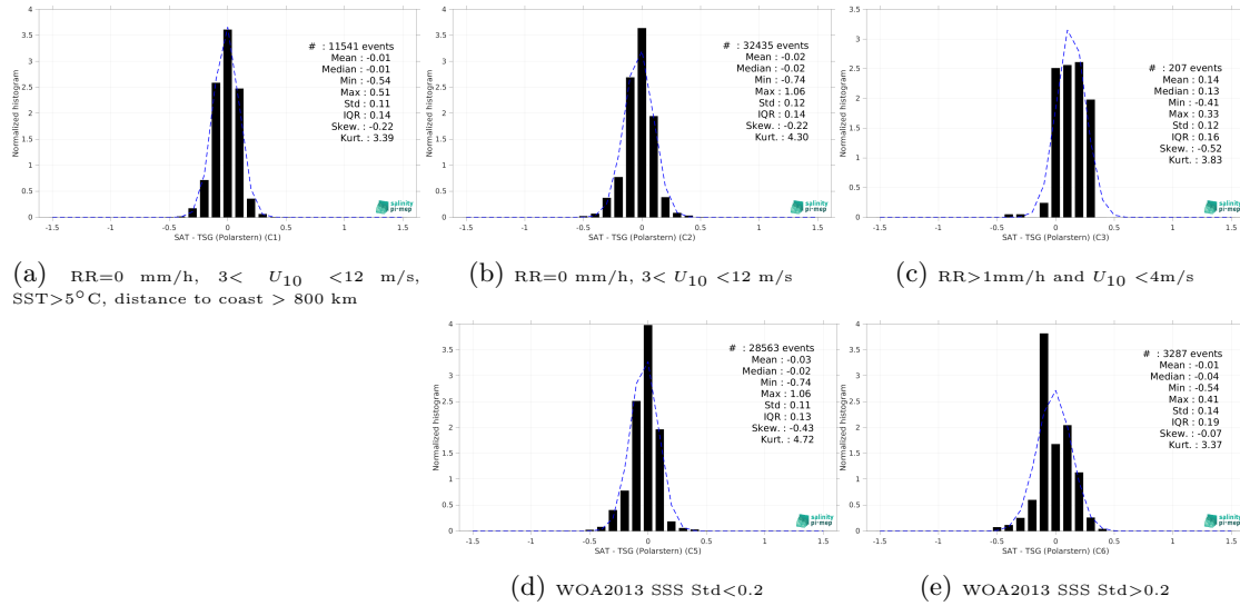
Figure 15: Normalized histogram of \Delta\text{SSS} (Aquarius SSS L4 OI v5 - Weekly (IPRC) - TSG (Polarstern)) for 5 different subdatasets corresponding to: RR=0 mm/h, 3 < U_{10} < 12 m/s, SST>5°C, distance to coast > 800 km (a), RR=0 mm/h, 3 < U_{10} < 12 m/s (b), RR>1mm/h and U_{10} < 4 m/s (c), WOA2013 SSS Std<0.2 (d), WOA2013 SSS Std>0.2 (e).
