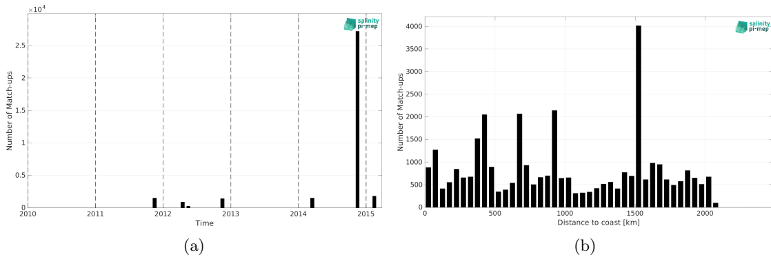
Figure 2: Number of match-ups between TSG (Polarstern) and Aquarius SSS L4 OI v5 - Weekly (IPRC) SSS as a function of time (a) and as function of the distance to coast (b) over the Tropical Atlantic Ocean Pi-MEP region and for the full satellite product period.
