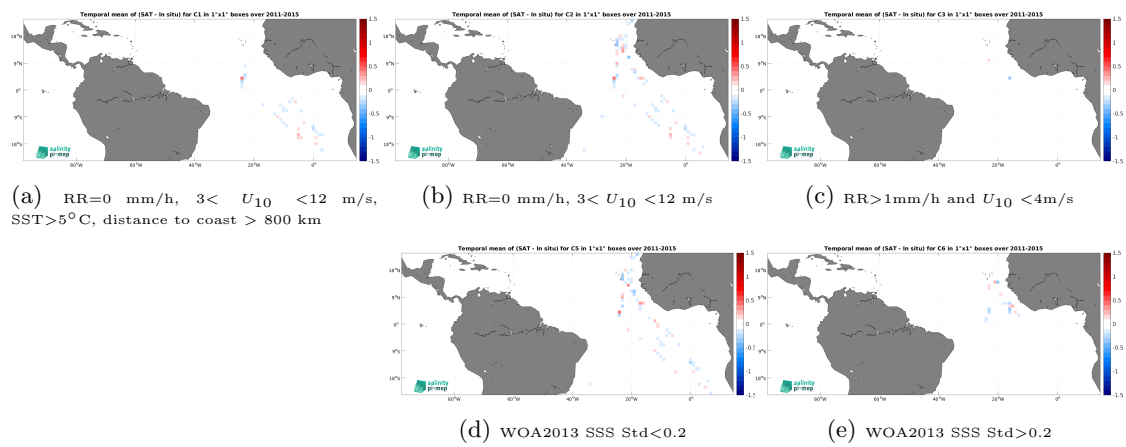
Figure 14: Temporal mean gridded over spatial boxes of size 1^\circ \times 1^\circ of \Delta SSS (Aquarius SSS L4 OI v5 - Weekly (IPRC) - TSG (Polarstern)) for 5 different subdatasets corresponding to:RR=0 mm/h, 3 < U_{10} < 12 m/s, SST > 5°C, distance to coast > 800 km (a), RR=0 mm/h, 3 < U_{10} < 12 m/s (b), RR > 1mm/h and U_{10} < 4 m/s (c), WOA2013 SSS Std < 0.2 (d), WOA2013 SSS Std > 0.2 (e).
