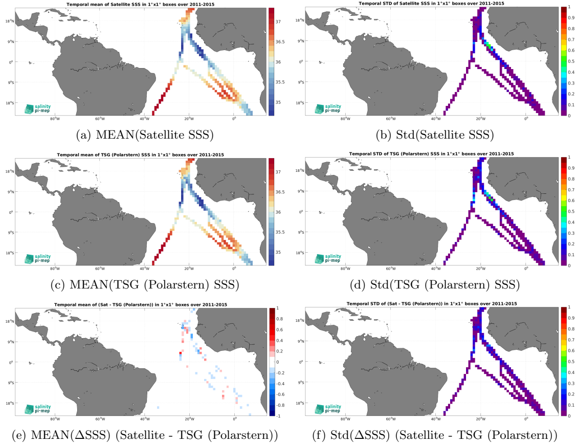
Figure 6: Temporal mean (left) and Std (right) of SSS from Aquarius SSS L4 OI v5 - Weekly (IPRC) (top), TSG (Polarstern) (middle), and of \Delta\text{SSS} (Satellite - TSG (Polarstern)). Only match-up pairs are used to generate these maps.
