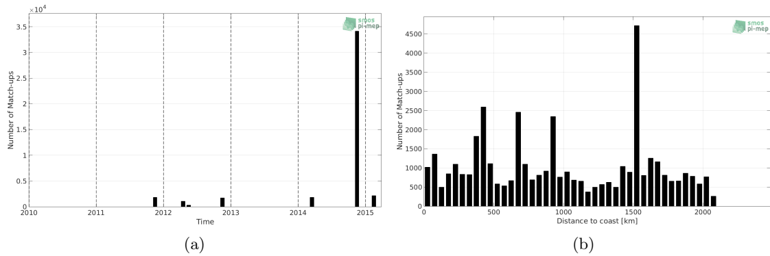
Figure 1: Number of match-ups between TSG-POLARSTERN and Aquarius-L4-IPRC-V5-WEEKLY SSS as a function of time (a) and as function of the distance to coast (b) over the Tropical Atlantic Ocean Pi-MEP region and for the full satellite product period.
