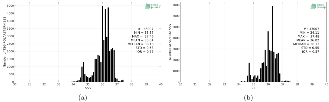
Figure 2: Histograms of SSS from TSG-POLARSTERN (a) and Aquarius-L4-IPRC-V5-WEEKLY (b) considering all match-up pairs per bins of 0.1 over the Tropical Atlantic Ocean Pi-MEP region and for the full satellite product period.
