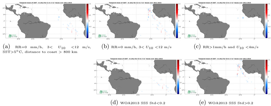
Figure 12: Temporal mean gridded over spatial boxes of size 1^\circ \times 1^\circ of \Delta SSS (Aquarius-L4-IPRC-V5-WEEKLY - TSG-POLARSTERN) for 5 different subdatasets corresponding to:RR=0 mm/h, 3 < U_{10} < 12 m/s, SST >5^\circ\text{C} , distance to coast > 800 km (a), RR=0 mm/h, 3 < U_{10} < 12 m/s (b), RR >1 mm/h and U_{10} < 4 m/s (c), WOA2013 SSS Std <0.2 (d), WOA2013 SSS Std >0.2 (e).
