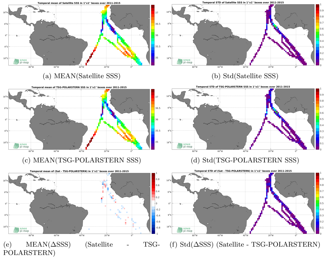
Figure 6: Temporal mean (left) and Std (right) of SSS from Aquarius-L4-IPRC-V5-WEEKLY (top), TSG-POLARSTERN (middle), and of \Delta SSS (Satellite - TSG-POLARSTERN). Only match-up pairs are used to generate these maps.
