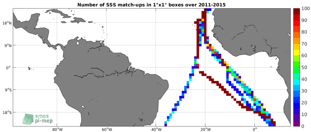
Figure 4: Number of SSS match-ups between TSG-POLARSTERN SSS and the Aquarius-L4-IPRC-V5-WEEKLY SSS product for the Tropical Atlantic Ocean Pi-MEP region over 1^\circ \times 1^\circ boxes and for the full satellite product period.
