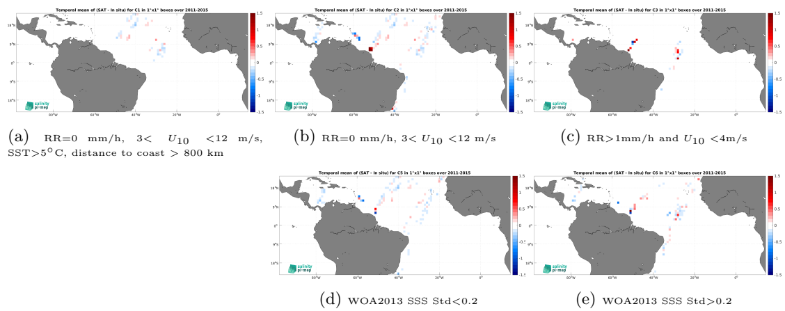
Figure 14: Temporal mean gridded over spatial boxes of size 1^\circ \times 1^\circ of \Delta SSS (Aquarius SSS L4 OI v5 - Weekly (IPRC) - TSG (LEGOS-DM)) for 5 different subdatasets corresponding to:RR=0 mm/h, 3 < U_{10} < 12 m/s, SST >5^\circ\text{C} , distance to coast > 800 km (a), RR=0 mm/h, 3 < U_{10} < 12 m/s (b), RR >1 mm/h and U_{10} < 4 m/s (c), WOA2013 SSS Std <0.2 (d), WOA2013 SSS Std >0.2 (e).
