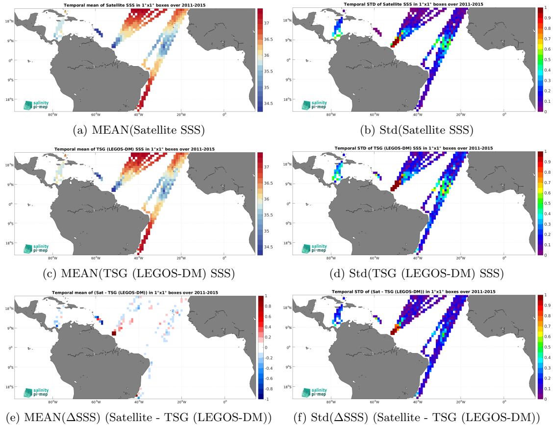
Figure 7: Temporal mean (left) and Std (right) of SSS from Aquarius SSS L4 OI v5 - Weekly (IPRC) (top), TSG (LEGOS-DM) (middle), and of \Delta\text{SSS} (Satellite - TSG (LEGOS-DM)). Only match-up pairs are used to generate these maps.
