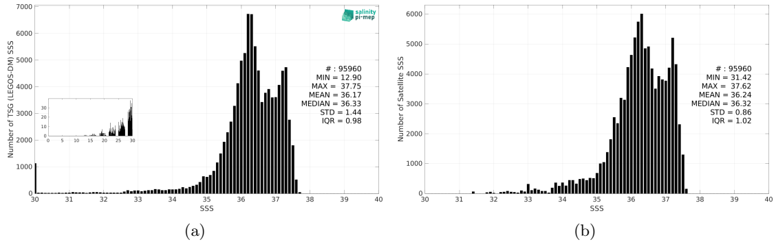
Figure 3: Histograms of SSS from TSG (LEGOS-DM) (a) and Aquarius SSS L4 OI v5 - Weekly (IPRC) (b) considering all match-up pairs per bins of 0.1 over the Tropical Atlantic Ocean Pi-MEP region and for the full satellite product period.
