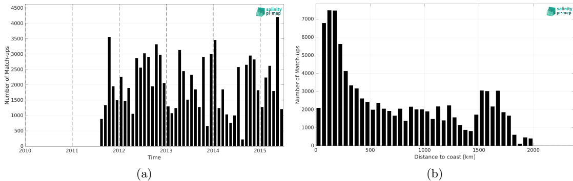
Figure 2: Number of match-ups between TSG (LEGOS-DM) and Aquarius SSS L4 OI v5 - Weekly (IPRC) SSS as a function of time (a) and as function of the distance to coast (b) over the Tropical Atlantic Ocean Pi-MEP region and for the full satellite product period.
