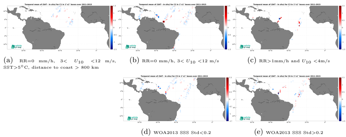
Figure 14: Temporal mean gridded over spatial boxes of size 1^\circ \times 1^\circ of \Delta SSS (Aquarius SSS L4 OI v5 - Weekly (IPRC) - TSG (LEGOS-DM)) for 5 different subdatasets corresponding to:RR=0 mm/h, 3 < U_{10} < 12 m/s, SST >5^\circ\text{C} , distance to coast > 800 km (a), RR=0 mm/h, 3 < U_{10} < 12 m/s (b), RR >1 mm/h and U_{10} < 4 m/s (c), WOA2013 SSS Std <0.2 (d), WOA2013 SSS Std >0.2 (e).
