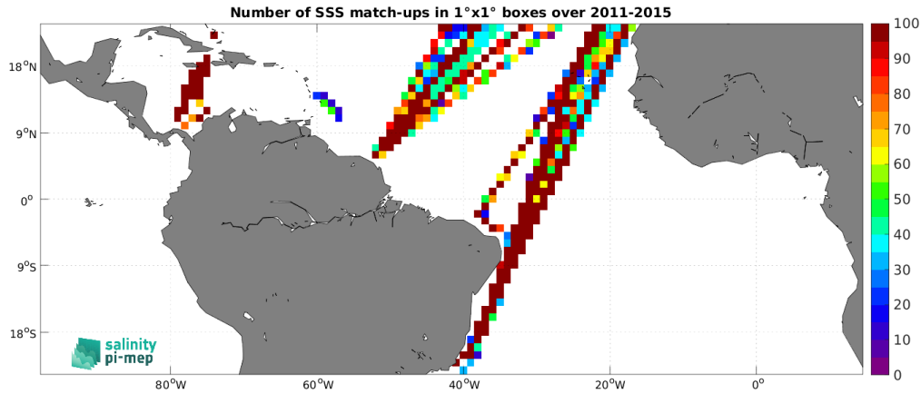
Figure 5: Number of SSS match-ups between TSG (LEGOS-DM) SSS and the Aquarius SSS L4 OI v5 - Weekly (IPRC) SSS product for the Tropical Atlantic Ocean Pi-MEP region over 1^\circ \times 1^\circ boxes and for the full satellite product period.
