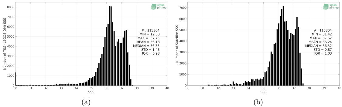
Figure 2: Histograms of SSS from TSG (LEGOS-DM) (a) and Aquarius SSS L4 OI v5 - Weekly (IPRC) (b) considering all match-up pairs per bins of 0.1 over the Tropical Atlantic Ocean Pi-MEP region and for the full satellite product period.
