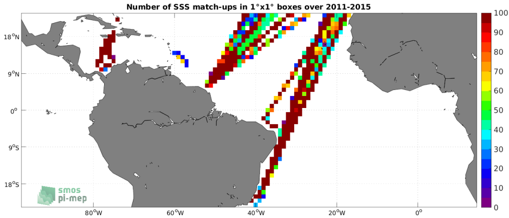
Figure 4: Number of SSS match-ups between TSG (LEGOS-DM) SSS and the Aquarius SSS L4 OI v5 - Weekly (IPRC) SSS product for the Tropical Atlantic Ocean Pi-MEP region over 1^\circ \times 1^\circ boxes and for the full satellite product period.
