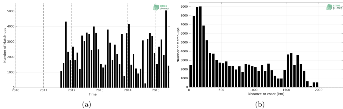
Figure 1: Number of match-ups between TSG (LEGOS-DM) and Aquarius SSS L4 OI v5 - Weekly (IPRC) SSS as a function of time (a) and as function of the distance to coast (b) over the Tropical Atlantic Ocean Pi-MEP region and for the full satellite product period.
