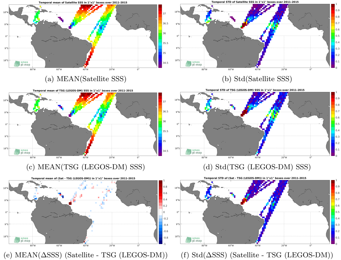
Figure 6: Temporal mean (left) and Std (right) of SSS from Aquarius SSS L4 OI v5 - Weekly (IPRC) (top), TSG (LEGOS-DM) (middle), and of \Delta SSS (Satellite - TSG (LEGOS-DM)). Only match-up pairs are used to generate these maps.
