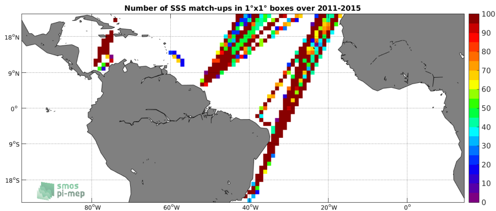
Figure 4: Number of SSS match-ups between TSG-LEGOS-DM SSS and the Aquarius-L4-IPRC-V5-WEEKLY SSS product for the Tropical Atlantic Ocean Pi-MEP region over 1^\circ \times 1^\circ boxes and for the full satellite product period.
