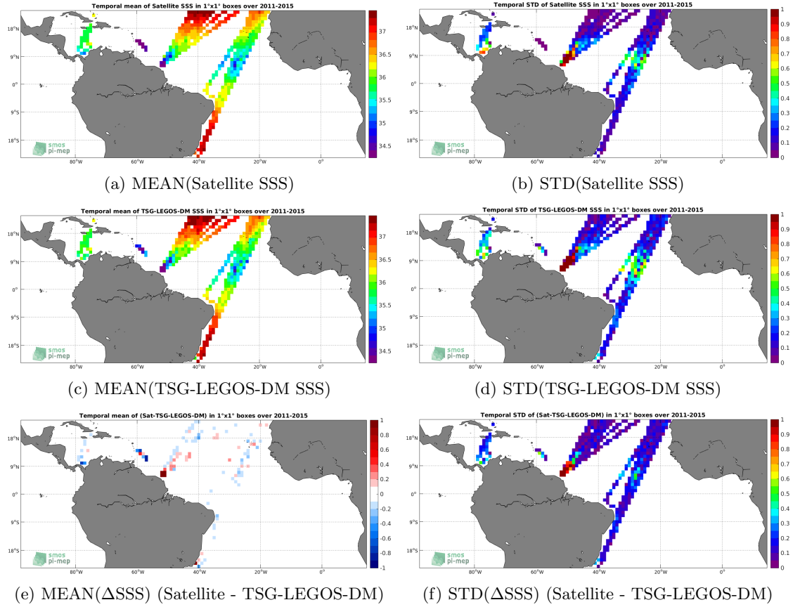
Figure 6: Temporal mean (left) and STD (right) of SSS from Aquarius-L4-IPRC-V5-WEEKLY (top), TSG-LEGOS-DM (middle), and of \Delta SSS (Satellite - TSG-LEGOS-DM). Only match-up pairs are used to generate these maps.
