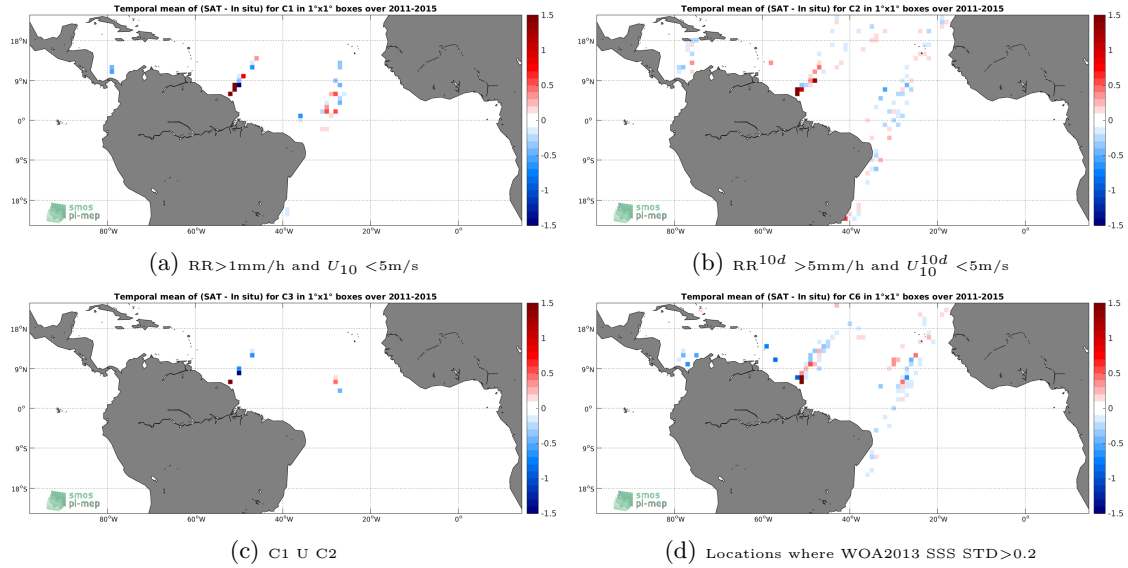
Figure 12: Temporal mean gridded over spatial boxes of size 1^\circ \times 1^\circ of \Delta SSS (Aquarius-L4-IPRC-V5-WEEKLY - TSG-LEGOS-DM) for 4 different subdatasets corresponding to: RR > 1\text{mm/h} and U_{10} < 5\text{m/s} (a), RR^{10d} > 5\text{mm/h} and U_{10}^{10d} < 5\text{m/s} (b), C1 U C2 (c), Locations where WOA2013 SSS STD > 0.2 (d).
