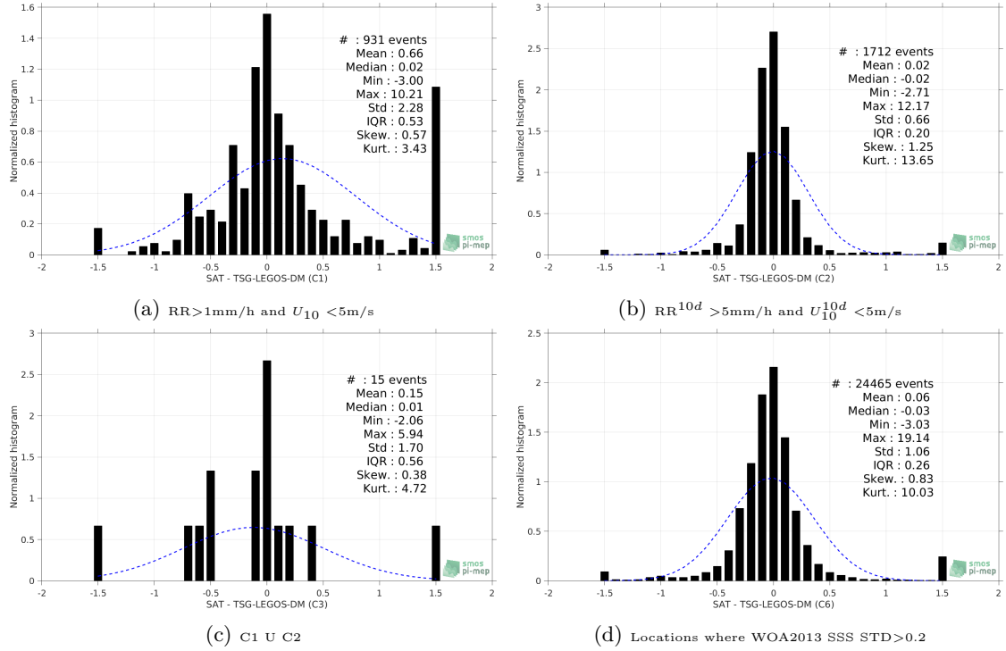
Figure 13: Normalized histogram of \Delta SSS (Aquarius-L4-IPRC-V5-WEEKLY - TSG-LEGOS-DM) for 6 different subdatasets corresponding to: RR > 1\text{mm/h} and U_{10} < 5\text{m/s} (a), RR^{10d} > 5\text{mm/h} and U_{10}^{10d} < 5\text{m/s} (b), C1 U C2 (c), Locations where WOA2013 SSS STD > 0.2 (d).
