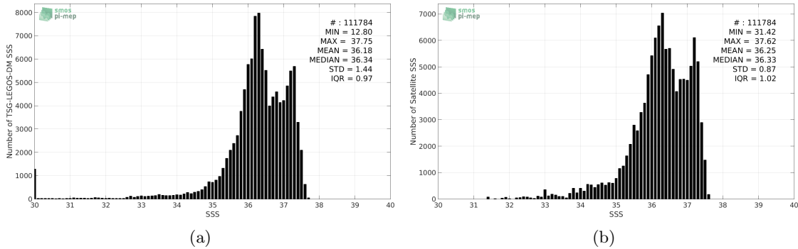
Figure 2: Histograms of SSS from TSG-LEGOS-DM (a) and Aquarius-L4-IPRC-V5-WEEKLY (b) considering all match-up pairs per bins of 0.1 over the Tropical Atlantic Ocean Pi-MEP region and for the full satellite product period.
