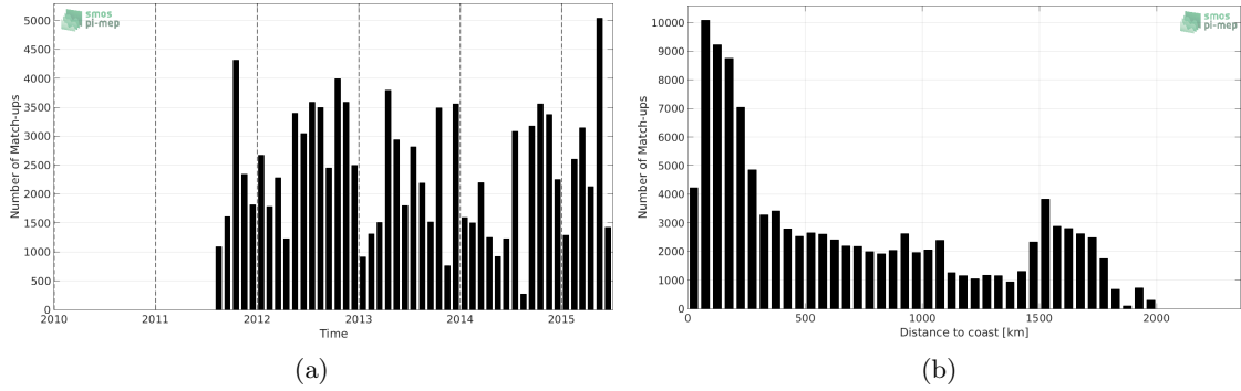
Figure 1: Number of match-ups between TSG-LEGOS-DM and Aquarius-L4-IPRC-V5-WEEKLY SSS as a function of time (a) and as function of the distance to coast (b) over the Tropical Atlantic Ocean Pi-MEP region and for the full satellite product period.
