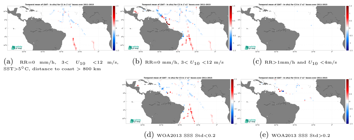
Figure 14: Temporal mean gridded over spatial boxes of size 1^\circ \times 1^\circ of \Delta SSS (Aquarius SSS L4 OI v5 - Weekly (IPRC) - TSG (GOSUD-Sailing-ship)) for 5 different subdatasets corresponding to:RR=0 mm/h, 3 < U_{10} < 12 m/s, SST >5^\circ\text{C} , distance to coast > 800 km (a), RR=0 mm/h, 3 < U_{10} < 12 m/s (b), RR >1 mm/h and U_{10} < 4 m/s (c), WOA2013 SSS Std <0.2 (d), WOA2013 SSS Std >0.2 (e).
