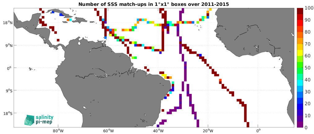
Figure 5: Number of SSS match-ups between TSG (GOSUD-Sailing-ship) SSS and the Aquarius SSS L4 OI v5 - Weekly (IPRC) SSS product for the Tropical Atlantic Ocean Pi-MEP region over 1^\circ \times 1^\circ boxes and for the full satellite product period.
