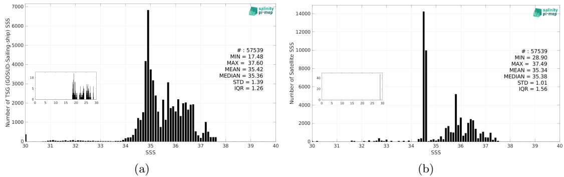
Figure 3: Histograms of SSS from TSG (GOSUD-Sailing-ship) (a) and Aquarius SSS L4 OI v5 - Weekly (IPRC) (b) considering all match-up pairs per bins of 0.1 over the Tropical Atlantic Ocean Pi-MEP region and for the full satellite product period.
