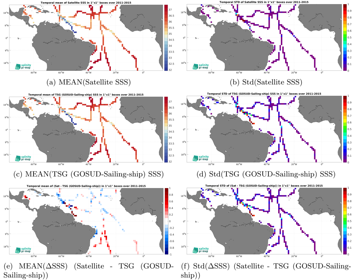
Figure 7: Temporal mean (left) and Std (right) of SSS from Aquarius SSS L4 OI v5 - Weekly (IPRC) (top), TSG (GOSUD-Sailing-ship) (middle), and of \Delta\text{SSS} (Satellite - TSG (GOSUD-Sailing-ship)). Only match-up pairs are used to generate these maps.
