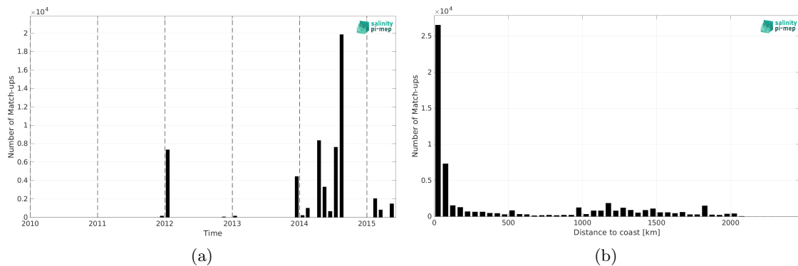
Figure 2: Number of match-ups between TSG (GOSUD-Sailing-ship) and Aquarius SSS L4 OI v5 - Weekly (IPRC) SSS as a function of time (a) and as function of the distance to coast (b) over the Tropical Atlantic Ocean Pi-MEP region and for the full satellite product period.
