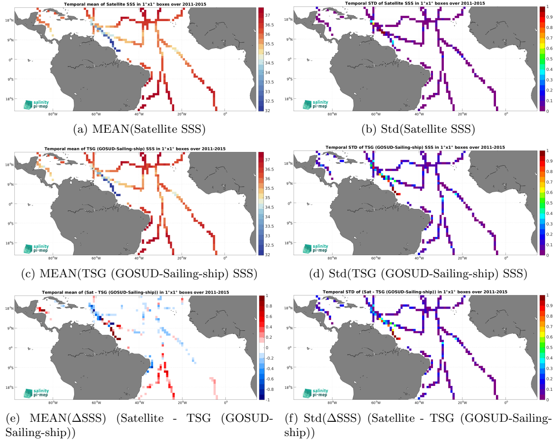
Figure 6: Temporal mean (left) and Std (right) of SSS from Aquarius SSS L4 OI v5 - Weekly (IPRC) (top), TSG (GOSUD-Sailing-ship) (middle), and of \Delta\text{SSS} (Satellite - TSG (GOSUD-Sailing-ship)). Only match-up pairs are used to generate these maps.
