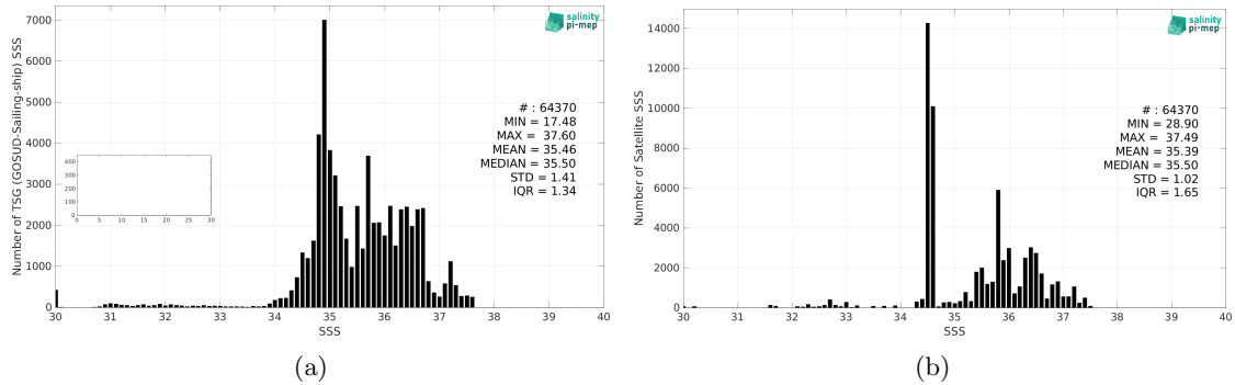
Figure 2: Histograms of SSS from TSG (GOSUD-Sailing-ship) (a) and Aquarius SSS L4 OI v5 - Weekly (IPRC) (b) considering all match-up pairs per bins of 0.1 over the Tropical Atlantic Ocean Pi-MEP region and for the full satellite product period.
