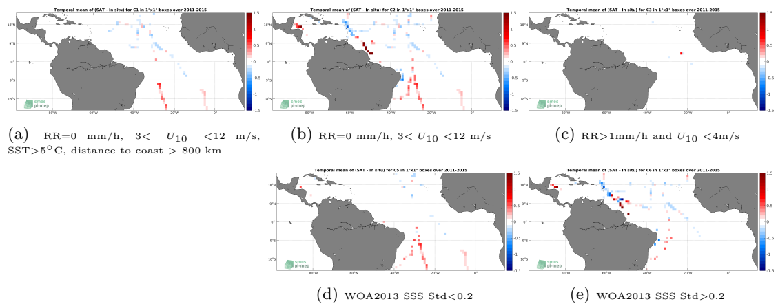
Figure 12: Temporal mean gridded over spatial boxes of size 1°x1° of \Delta SSS (Aquarius SSS L4 OI v5 - Weekly (IPRC) - TSG (GOSUD-Sailing-ship)) for 5 different subdatasets corresponding to:RR=0 mm/h, 3 < U_{10} < 12 m/s, SST>5°C, distance to coast > 800 km (a), RR=0 mm/h, 3 < U_{10} < 12 m/s (b), RR>1mm/h and U_{10} < 4m/s (c), WOA2013 SSS Std<0.2 (d), WOA2013 SSS Std>0.2 (e).
