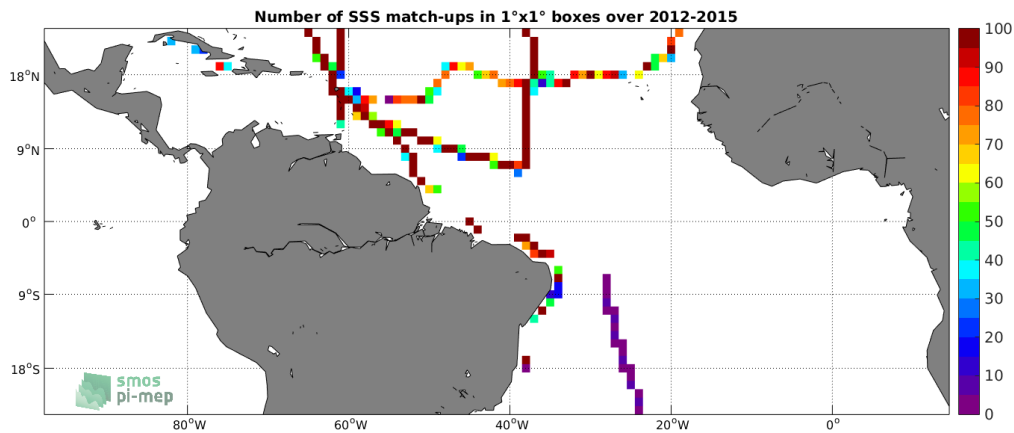
Figure 4: Number of SSS match-ups between TSG-GOSUD-Sailing-ship SSS and the Aquarius-L4-IPRC-V5-WEEKLY SSS product for the Tropical Atlantic Ocean Pi-MEP region over 1^\circ \times 1^\circ boxes and for the full satellite product period.
