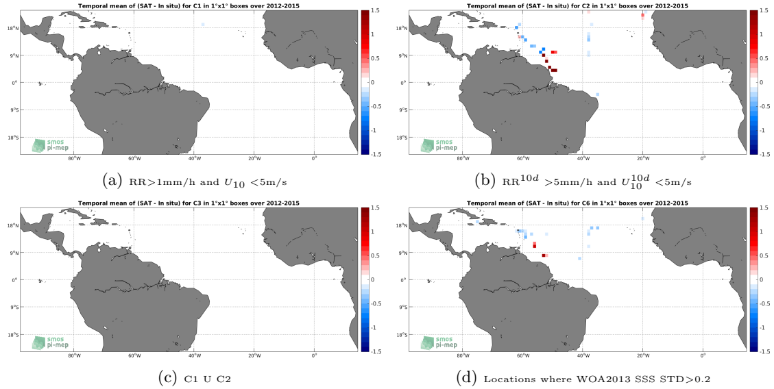
Figure 12: Temporal mean gridded over spatial boxes of size 1^\circ \times 1^\circ of \Delta SSS (Aquarius-L4-IPRC-V5-WEEKLY - TSG-GOSUD-Sailing-ship) for 4 different subdatasets corresponding to: RR > 1mm/h and U_{10} < 5\text{m/s} (a), RR^{10d} > 5\text{mm/h} and U_{10}^{10d} < 5\text{m/s} (b), C1 U C2 (c), Locations where WOA2013 SSS STD > 0.2 (d).
