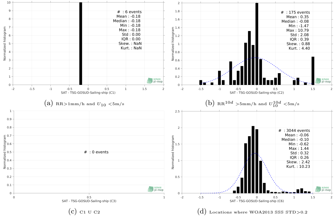
Figure 13: Normalized histogram of \Delta\text{SSS} (Aquarius-L4-IPRC-V5-WEEKLY - TSG-GOSUD-Sailing-ship) for 6 different subdatasets corresponding to: RR > 1mm/h and U_{10} < 5\text{m/s} (a), RR^{10d} > 5\text{mm/h} and U_{10}^{10d} < 5\text{m/s} (b), C1 U C2 (c), Locations where WOA2013 SSS STD > 0.2 (d).
