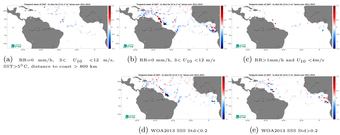
Figure 14: Temporal mean gridded over spatial boxes of size 1^\circ \times 1^\circ of \Delta SSS (Aquarius SSS L4 OI v5 - Weekly (IPRC) - TSG (GOSUD-Research-vessel)) for 5 different subdatasets corresponding to:RR=0 mm/h, 3 < U_{10} < 12 m/s, SST >5^\circ\text{C} , distance to coast > 800 km (a), RR=0 mm/h, 3 < U_{10} < 12 m/s (b), RR >1 mm/h and U_{10} < 4 m/s (c), WOA2013 SSS Std <0.2 (d), WOA2013 SSS Std >0.2 (e).
