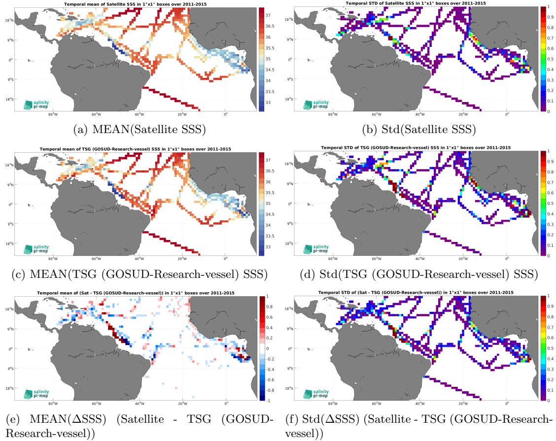
Figure 7: Temporal mean (left) and Std (right) of SSS from Aquarius SSS L4 OI v5 - Weekly (IPRC) (top), TSG (GOSUD-Research-vessel) (middle), and of \Delta\text{SSS} (Satellite - TSG (GOSUD-Research-vessel)). Only match-up pairs are used to generate these maps.
