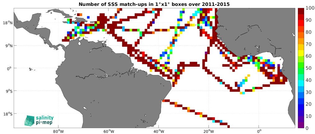
Figure 5: Number of SSS match-ups between TSG (GOSUD-Research-vessel) SSS and the Aquarius SSS L4 OI v5 - Weekly (IPRC) SSS product for the Tropical Atlantic Ocean Pi-MEP region over 1^\circ \times 1^\circ boxes and for the full satellite product period.
