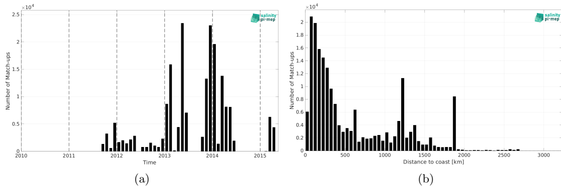
Figure 2: Number of match-ups between TSG (GOSUD-Research-vessel) and Aquarius SSS L4 OI v5 - Weekly (IPRC) SSS as a function of time (a) and as function of the distance to coast (b) over the Tropical Atlantic Ocean Pi-MEP region and for the full satellite product period.
