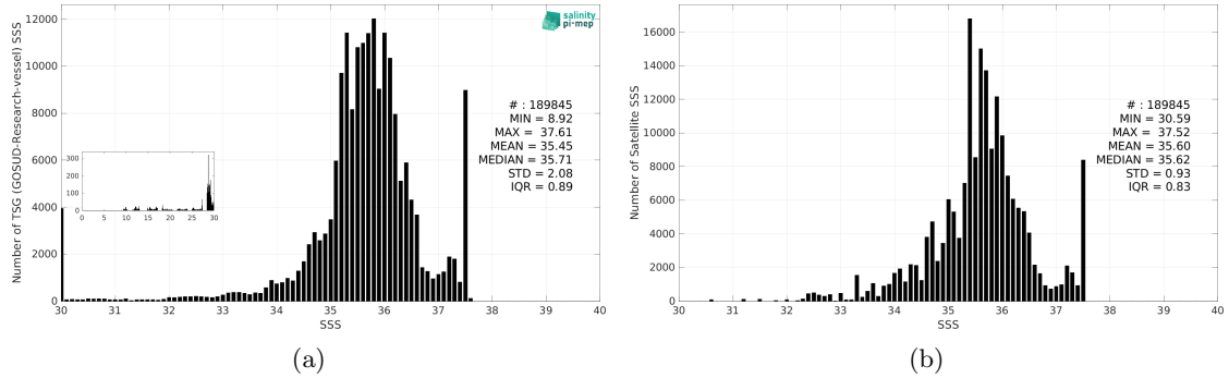
Figure 3: Histograms of SSS from TSG (GOSUD-Research-vessel) (a) and Aquarius SSS L4 OI v5 - Weekly (IPRC) (b) considering all match-up pairs per bins of 0.1 over the Tropical Atlantic Ocean Pi-MEP region and for the full satellite product period.
