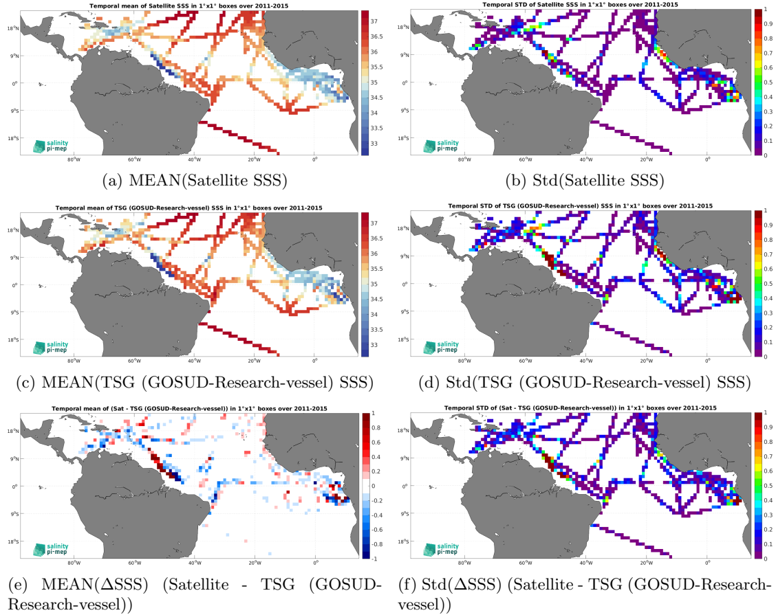
Figure 6: Temporal mean (left) and Std (right) of SSS from Aquarius SSS L4 OI v5 - Weekly (IPRC) (top), TSG (GOSUD-Research-vessel) (middle), and of \Delta\text{SSS} (Satellite - TSG (GOSUD-Research-vessel)). Only match-up pairs are used to generate these maps.
