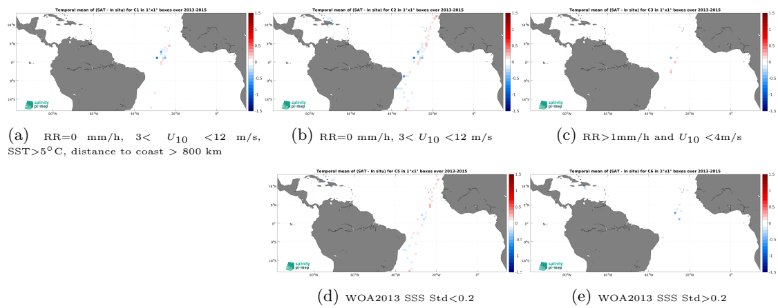
Figure 14: Temporal mean gridded over spatial boxes of size 1^\circ \times 1^\circ of \Delta SSS (Aquarius SSS L4 OI v5 - Weekly (IPRC) - TSG (CSIC-UTM)) for 5 different subdatasets corresponding to:RR=0 mm/h, 3 < U_{10} < 12 m/s, SST >5^\circ\text{C} , distance to coast > 800 km (a), RR=0 mm/h, 3 < U_{10} < 12 m/s (b), RR >1 mm/h and U_{10} < 4 m/s (c), WOA2013 SSS Std <0.2 (d), WOA2013 SSS Std >0.2 (e).
