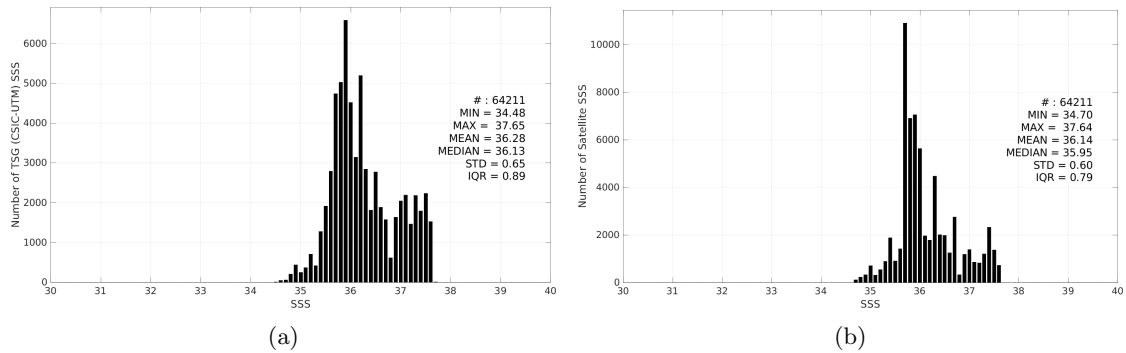
Figure 3: Histograms of SSS from TSG (CSIC-UTM) (a) and Aquarius SSS L4 OI v5 - Weekly (IPRC) (b) considering all match-up pairs per bins of 0.1 over the Tropical Atlantic Ocean Pi-MEP region and for the full satellite product period.
