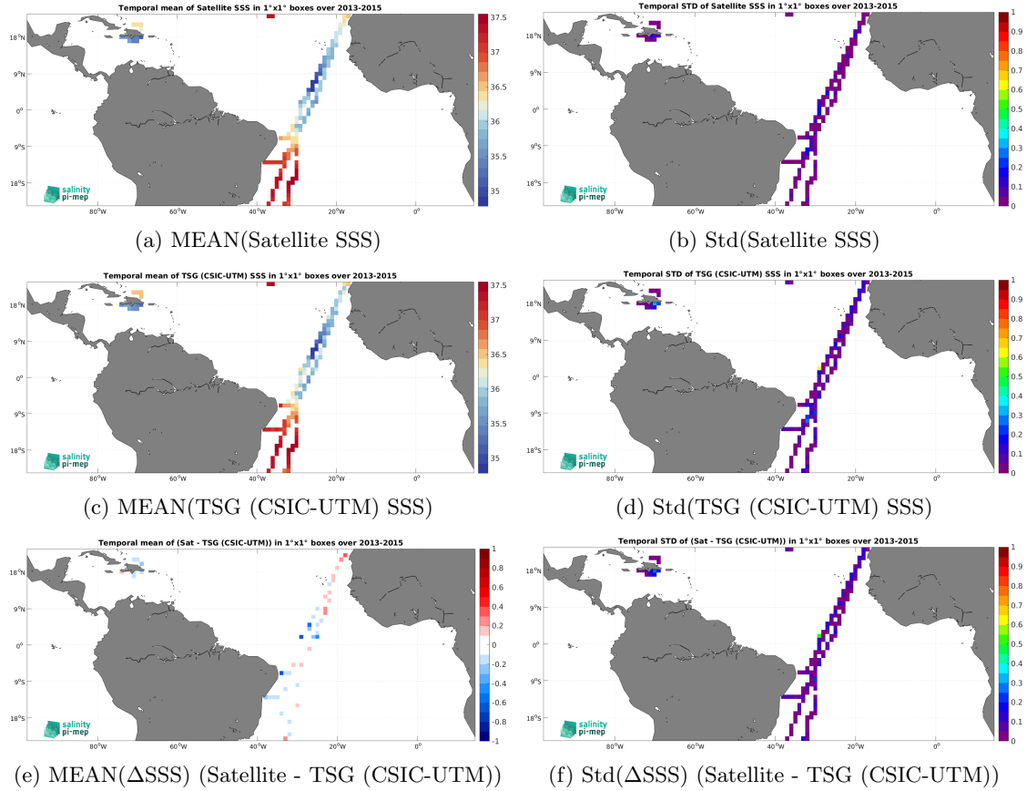
Figure 7: Temporal mean (left) and Std (right) of SSS from Aquarius SSS L4 OI v5 - Weekly (IPRC) (top), TSG (CSIC-UTM) (middle), and of \Delta\text{SSS} (Satellite - TSG (CSIC-UTM)). Only match-up pairs are used to generate these maps.
