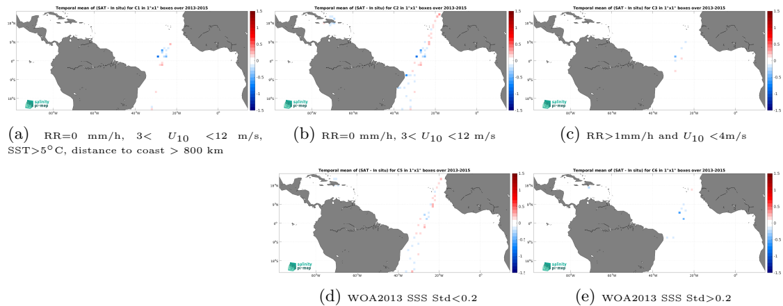
Figure 12: Temporal mean gridded over spatial boxes of size 1^\circ \times 1^\circ of \Delta SSS (Aquarius SSS L4 OI v5 - Weekly (IPRC) - TSG (CSIC-UTM)) for 5 different subdatasets corresponding to:RR=0 mm/h, 3 < U_{10} < 12 m/s, SST >5^\circ\text{C} , distance to coast > 800 km (a), RR=0 mm/h, 3 < U_{10} < 12 m/s (b), RR >1 mm/h and U_{10} < 4 m/s (c), WOA2013 SSS Std <0.2 (d), WOA2013 SSS Std >0.2 (e).
