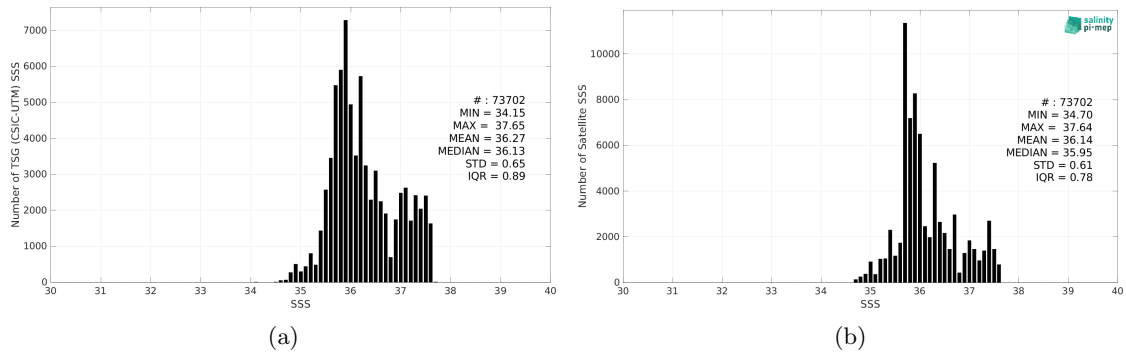
Figure 2: Histograms of SSS from TSG (CSIC-UTM) (a) and Aquarius SSS L4 OI v5 - Weekly (IPRC) (b) considering all match-up pairs per bins of 0.1 over the Tropical Atlantic Ocean Pi-MEP region and for the full satellite product period.
