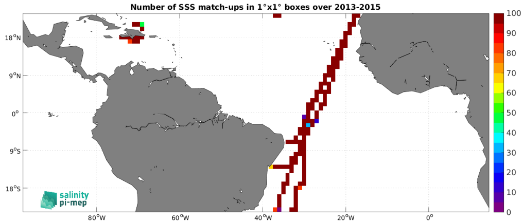
Figure 4: Number of SSS match-ups between TSG (CSIC-UTM) SSS and the Aquarius SSS L4 OI v5 - Weekly (IPRC) SSS product for the Tropical Atlantic Ocean Pi-MEP region over 1^\circ \times 1^\circ boxes and for the full satellite product period.
