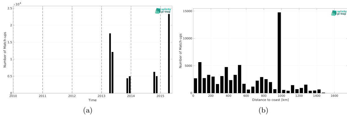
Figure 1: Number of match-ups between TSG (CSIC-UTM) and Aquarius SSS L4 OI v5 - Weekly (IPRC) SSS as a function of time (a) and as function of the distance to coast (b) over the Tropical Atlantic Ocean Pi-MEP region and for the full satellite product period.
