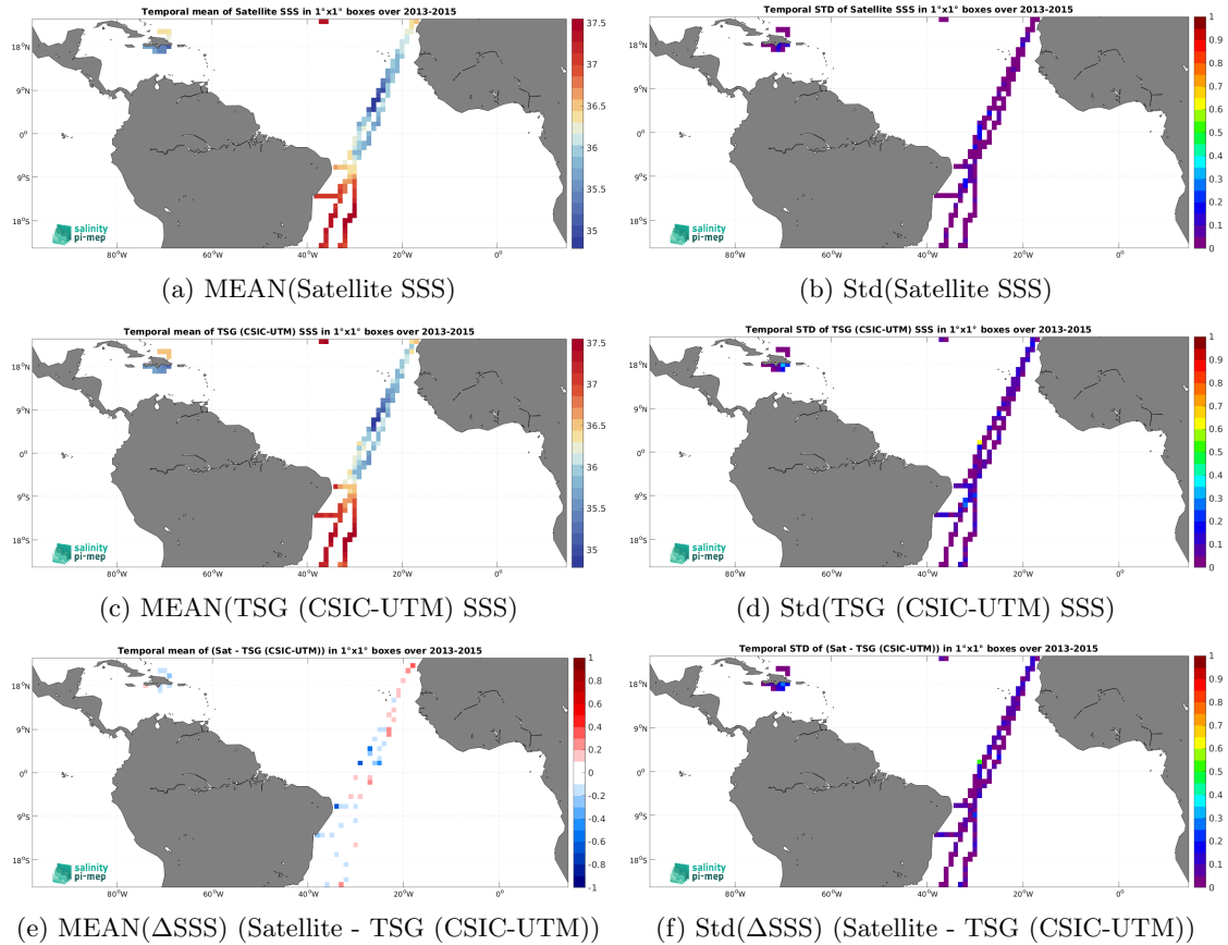
Figure 6: Temporal mean (left) and Std (right) of SSS from Aquarius SSS L4 OI v5 - Weekly (IPRC) (top), TSG (CSIC-UTM) (middle), and of \Delta\text{SSS} (Satellite - TSG (CSIC-UTM)). Only match-up pairs are used to generate these maps.
