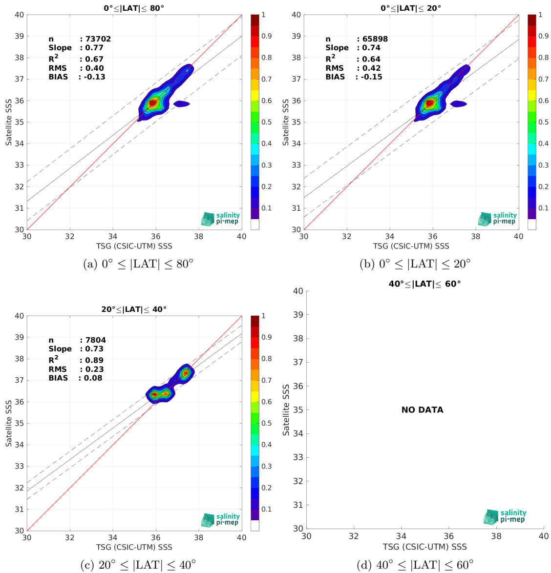
Figure 9: Contour maps of the concentration of Aquarius SSS L4 OI v5 - Weekly (IPRC) SSS (y-axis) versus TSG (CSIC-UTM) SSS (x-axis) at match-up pairs for different latitude bands. For each plot, the red line shows x=y . The black thin and dashed lines indicate a linear fit through the data cloud and the \pm 95\% confidence levels, respectively. The number match-up pairs n , the slope and R^2 coefficient of the linear fit, the root mean square (RMS) and the mean bias between satellite and in situ data are indicated for each latitude band in each plots.
