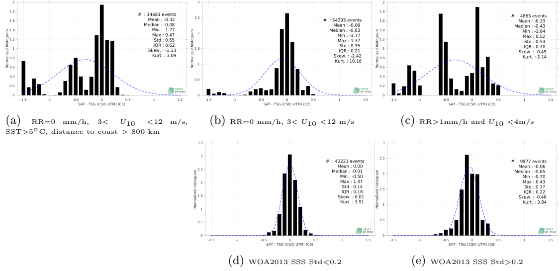
Figure 13: Normalized histogram of \Delta SSS (Aquarius SSS L4 OI v5 - Weekly (IPRC) - TSG (CSIC-UTM)) for 5 different subdatasets corresponding to: RR=0 mm/h, 3 < U_{10} < 12 m/s, SST>5°C, distance to coast > 800 km (a), RR=0 mm/h, 3 < U_{10} < 12 m/s (b), RR>1mm/h and U_{10} < 4 m/s (c), WOA2013 SSS Std<0.2 (d), WOA2013 SSS Std>0.2 (e).
