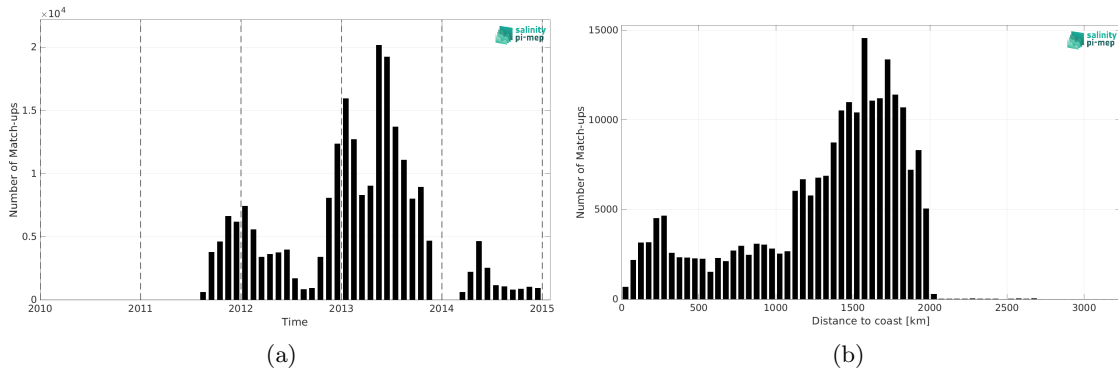
Figure 2: Number of match-ups between Surface drifters and Aquarius SSS L4 OI v5 - Weekly (IPRC) SSS as a function of time (a) and as function of the distance to coast (b) over the Tropical Atlantic Ocean Pi-MEP region and for the full satellite product period.
