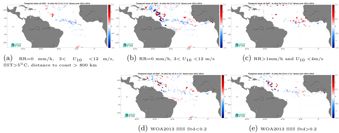
Figure 13: Temporal mean gridded over spatial boxes of size 1^\circ \times 1^\circ of \Delta\text{SSS} (Aquarius SSS L4 OI v5 - Weekly (IPRC) - Surface drifters) for 5 different subdatasets corresponding to:RR=0 mm/h, 3 < U_{10} < 12 m/s, SST >5^\circ\text{C} , distance to coast > 800 km (a), RR=0 mm/h, 3 < U_{10} < 12 m/s (b), RR >1 mm/h and U_{10} < 4 m/s (c), WOA2013 SSS Std <0.2 (d), WOA2013 SSS Std >0.2 (e).
