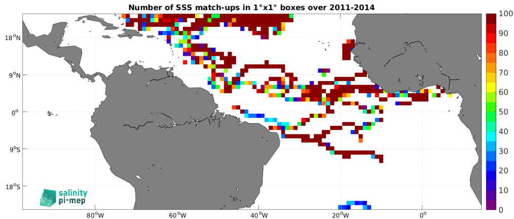
Figure 4: Number of SSS match-ups between Surface drifters SSS and the Aquarius SSS L4 OI v5 - Weekly (IPRC) SSS product for the Tropical Atlantic Ocean Pi-MEP region over 1^\circ \times 1^\circ boxes and for the full satellite product period.
