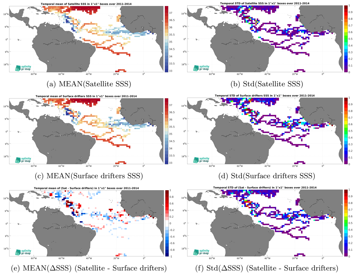
Figure 6: Temporal mean (left) and Std (right) of SSS from Aquarius SSS L4 OI v5 - Weekly (IPRC) (top), Surface drifters (middle), and of \Delta SSS (Satellite - Surface drifters). Only match-up pairs are used to generate these maps.
