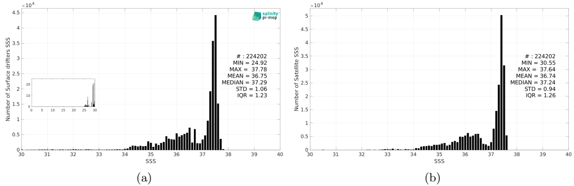
Figure 3: Histograms of SSS from Surface drifters (a) and Aquarius SSS L4 OI v5 - Weekly (IPRC) (b) considering all match-up pairs per bins of 0.1 over the Tropical Atlantic Ocean Pi-MEP region and for the full satellite product period.
